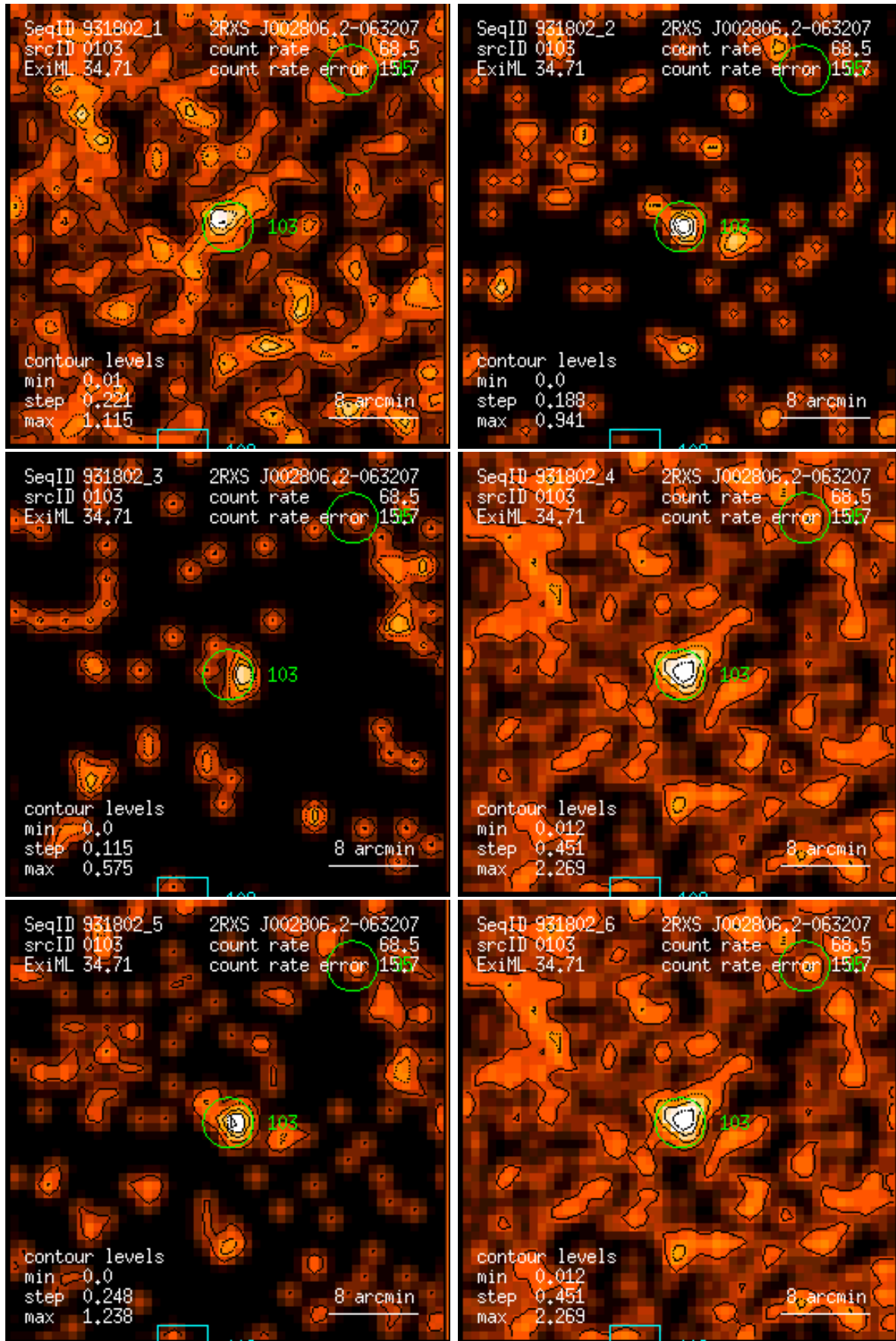
Figure 103: RASS 931802: detection 0103: band rate images, Gaussian filter: (1) PSPC channels 11 – 41, (2) 52 – 90, (3) 91 – 201, (4) 11 – 235, (5) 52 – 201, (6) 11 – 201. Broad band rates in counts/ks. Band rate contour levels in counts/ks/arcmin 2 .
