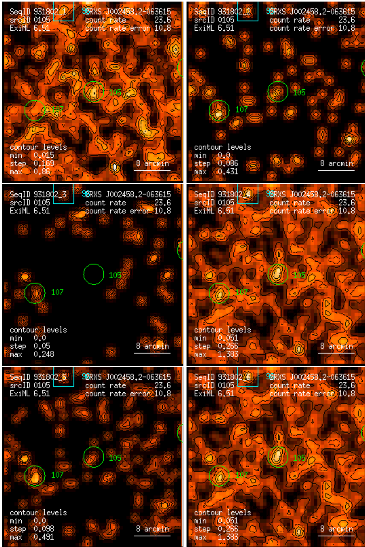
Figure 105: RASS 931802: detection 0105: band rate images, Gaussian filter: (1) PSPC channels 11 – 41, (2) 52 – 90, (3) 91 – 201, (4) 11 – 235, (5) 52 – 201, (6) 11 – 201. Broad band rates in counts/ks. Band rate contour levels in counts/ks/arcmin 2 .
