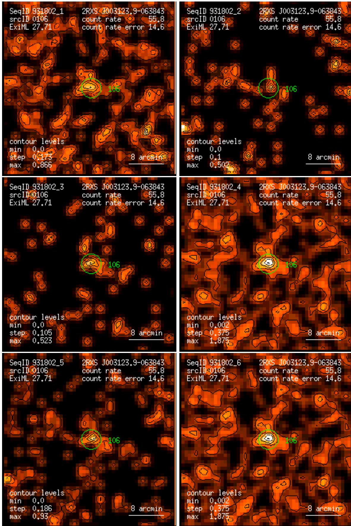
Figure 106: RASS 931802: detection 0106: band rate images, Gaussian filter: (1) PSPC channels 11 – 41, (2) 52 – 90, (3) 91 – 201, (4) 11 – 235, (5) 52 – 201, (6) 11 – 201. Broad band rates in counts/ks. Band rate contour levels in counts/ks/arcmin 2 .
