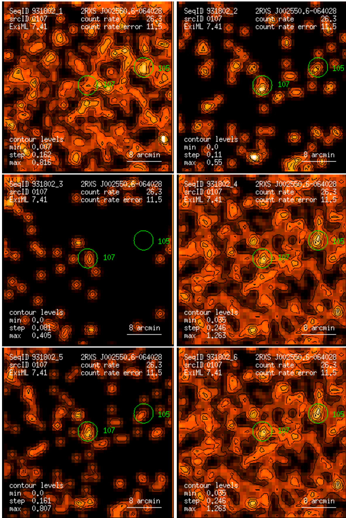
Figure 107: RASS 931802: detection 0107: band rate images, Gaussian filter: (1) PSPC channels 11 – 41, (2) 52 – 90, (3) 91 – 201, (4) 11 – 235, (5) 52 – 201, (6) 11 – 201. Broad band rates in counts/ks. Band rate contour levels in counts/ks/arcmin 2 .
