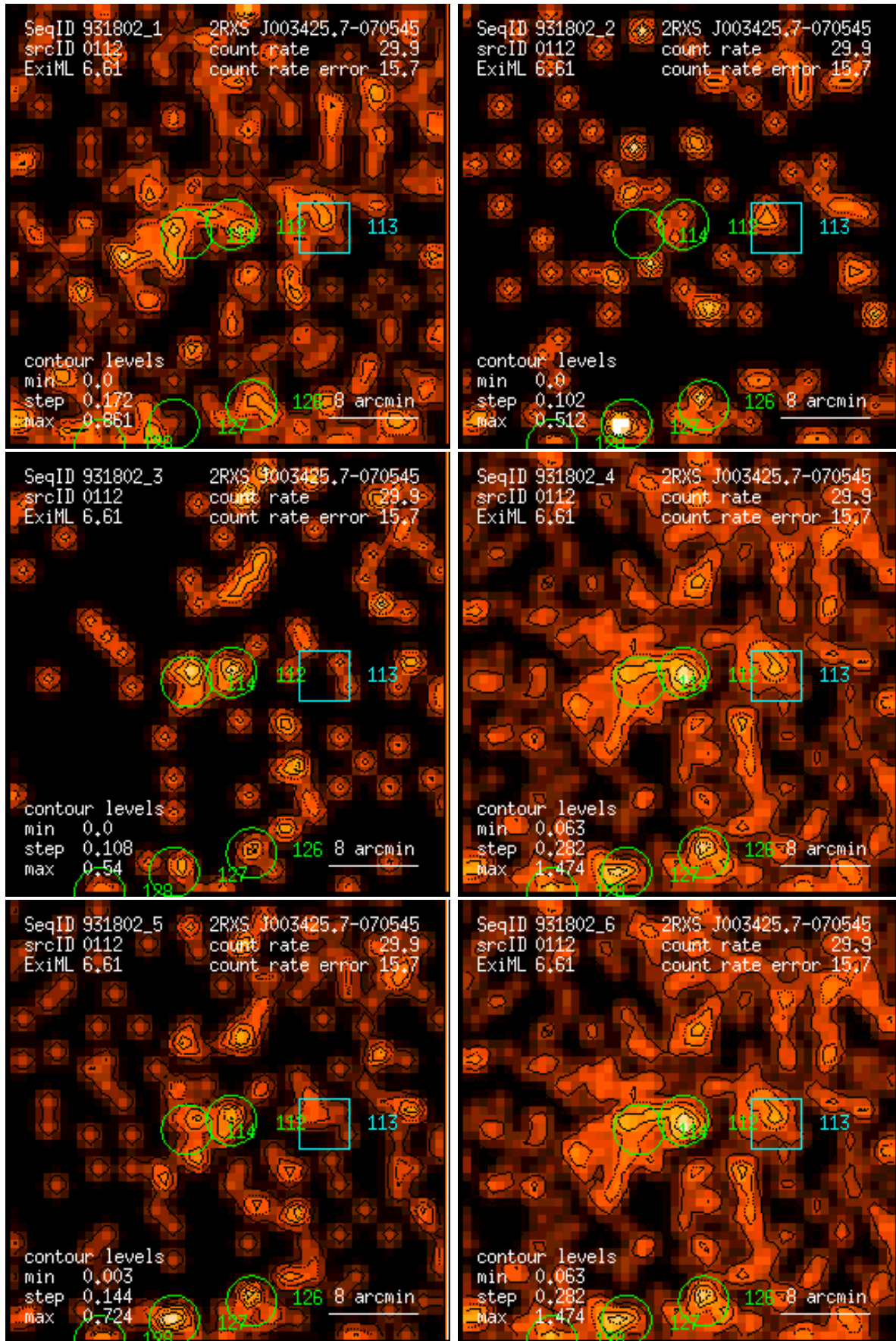
Figure 112: RASS 931802: detection 0112: band rate images, Gaussian filter: (1) PSPC channels 11 – 41, (2) 52 – 90, (3) 91 – 201, (4) 11 – 235, (5) 52 – 201, (6) 11 – 201. Broad band rates in counts/ks. Band rate contour levels in counts/ks/arcmin 2 .
