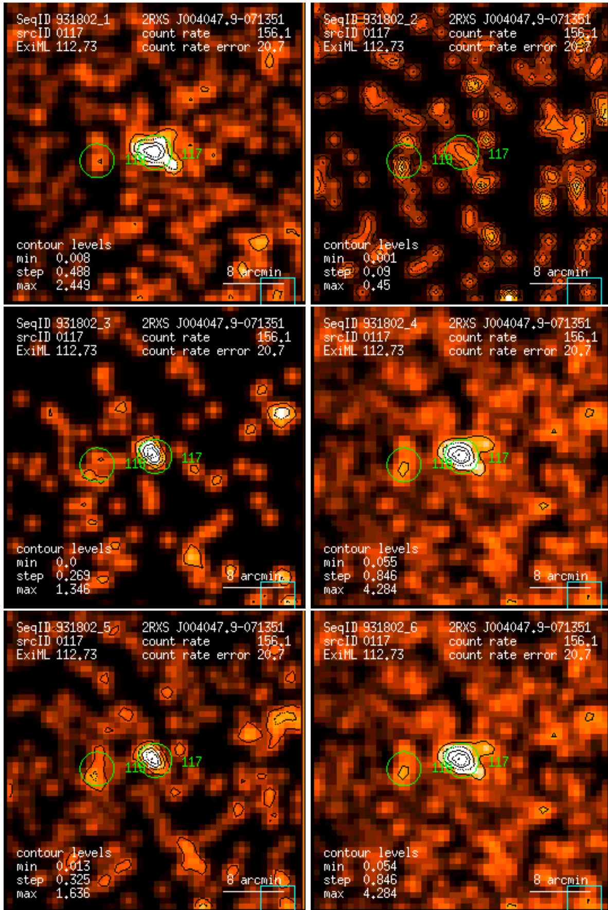
Figure 117: RASS 931802: detection 0117: band rate images, Gaussian filter: (1) PSPC channels 11 – 41, (2) 52 – 90, (3) 91 – 201, (4) 11 – 235, (5) 52 – 201, (6) 11 – 201. Broad band rates in counts/ks. Band rate contour levels in counts/ks/arcmin 2 .
