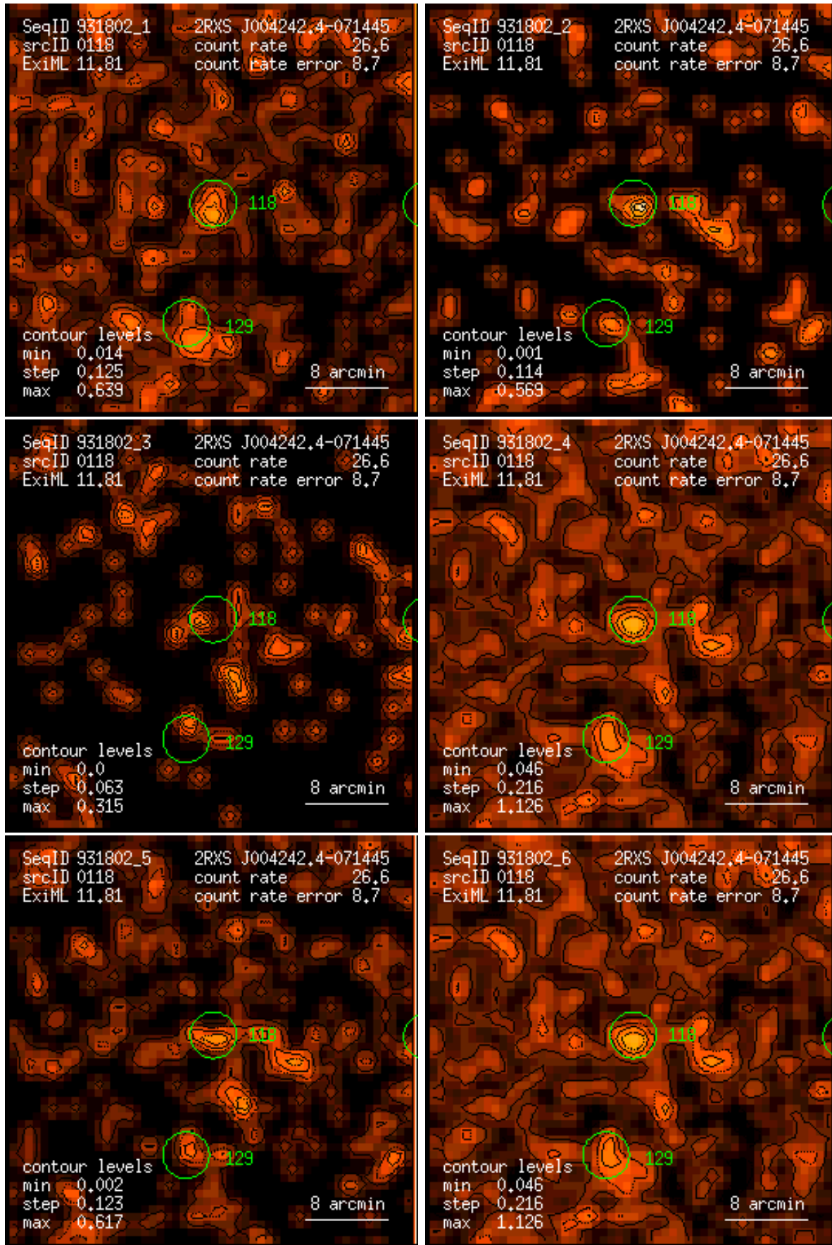
Figure 118: RASS 931802: detection 0118: band rate images, Gaussian filter: (1) PSPC channels 11 – 41, (2) 52 – 90, (3) 91 – 201, (4) 11 – 235, (5) 52 – 201, (6) 11 – 201. Broad band rates in counts/ks. Band rate contour levels in counts/ks/arcmin 2 .
