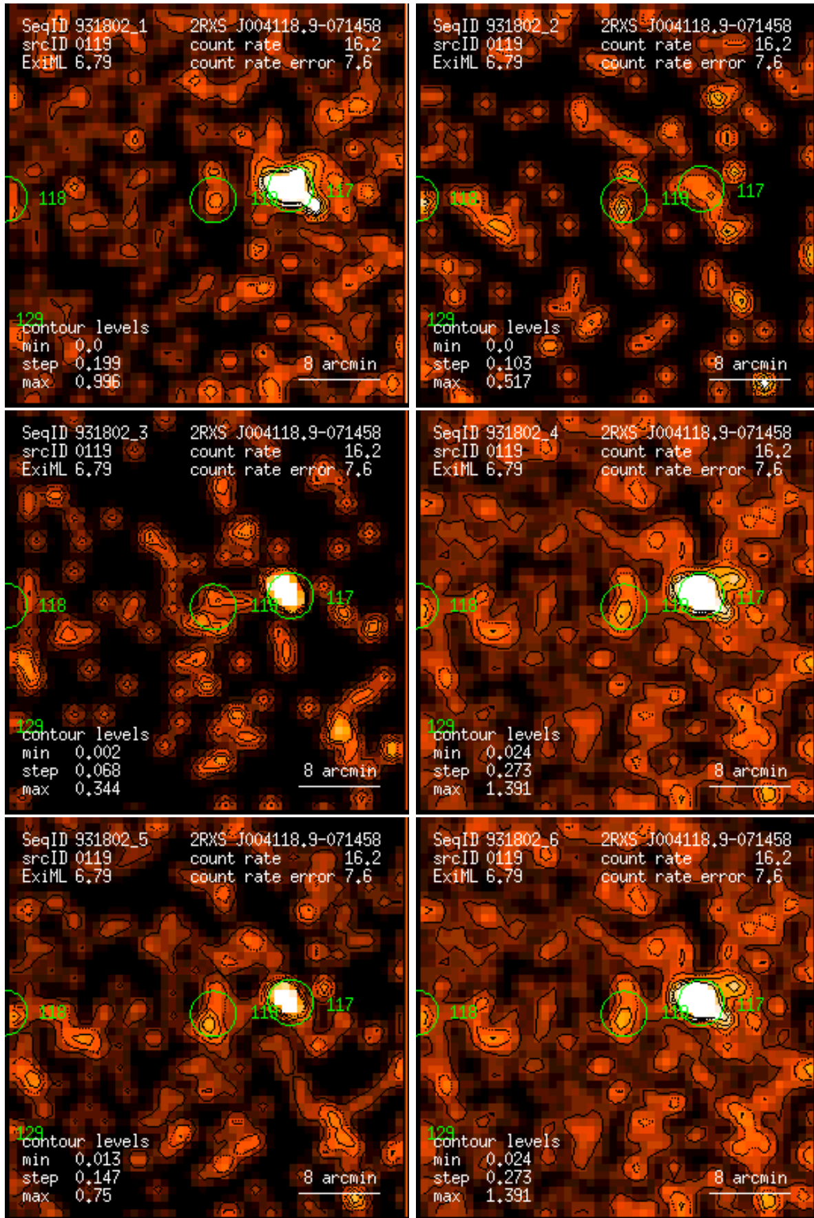
Figure 119: RASS 931802: detection 0119: band rate images, Gaussian filter: (1) PSPC channels 11 – 41, (2) 52 – 90, (3) 91 – 201, (4) 11 – 235, (5) 52 – 201, (6) 11 – 201. Broad band rates in counts/ks. Band rate contour levels in counts/ks/arcmin 2 .
