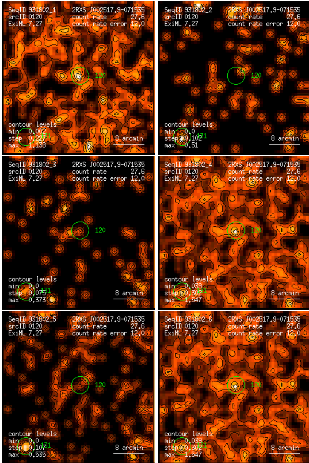
Figure 120: RASS 931802: detection 0120: band rate images, Gaussian filter: (1) PSPC channels 11 – 41, (2) 52 – 90, (3) 91 – 201, (4) 11 – 235, (5) 52 – 201, (6) 11 – 201. Broad band rates in counts/ks. Band rate contour levels in counts/ks/arcmin 2 .
