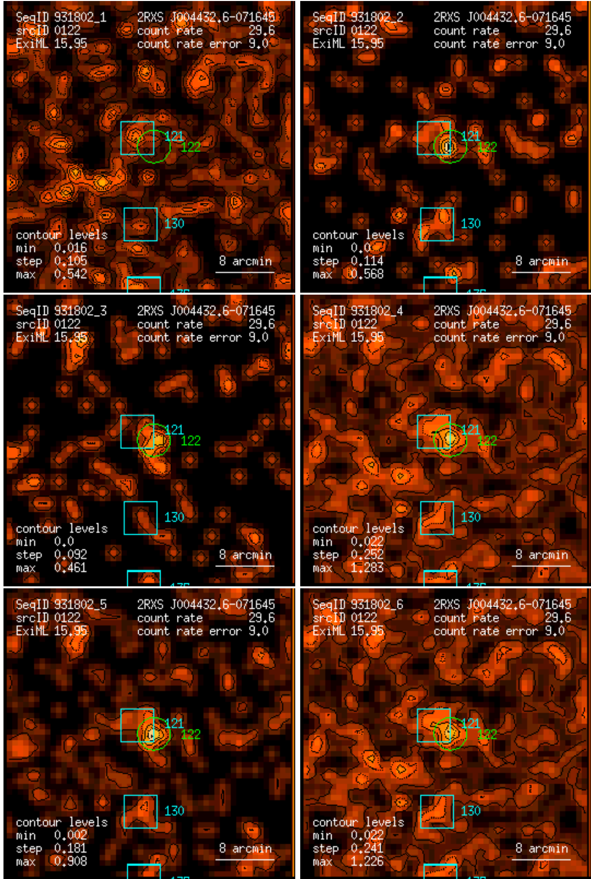
Figure 122: RASS 931802: detection 0122: band rate images, Gaussian filter: (1) PSPC channels 11 – 41, (2) 52 – 90, (3) 91 – 201, (4) 11 – 235, (5) 52 – 201, (6) 11 – 201. Broad band rates in counts/ks. Band rate contour levels in counts/ks/arcmin 2 .
