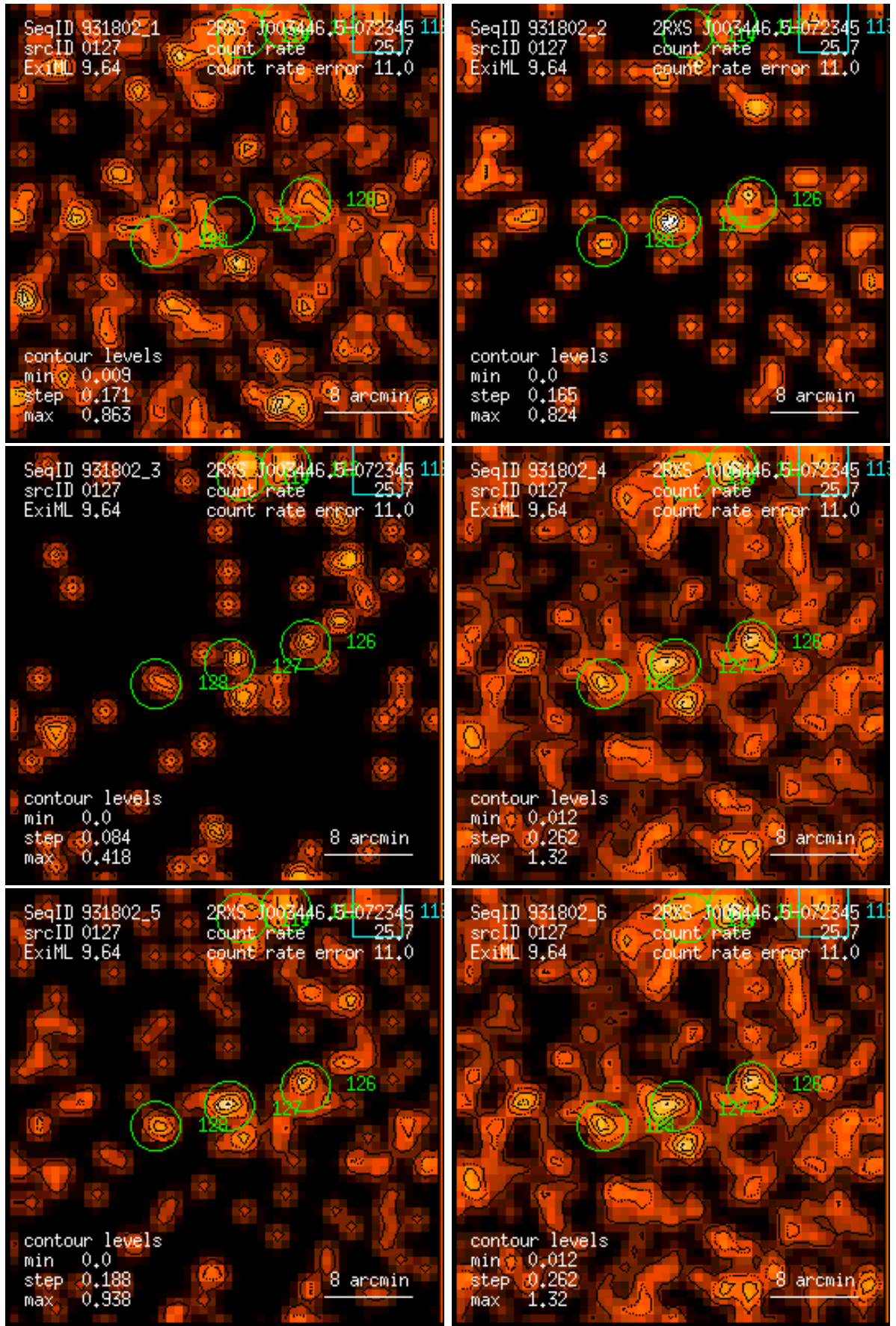
Figure 127: RASS 931802: detection 0127: band rate images, Gaussian filter: (1) PSPC channels 11 – 41, (2) 52 – 90, (3) 91 – 201, (4) 11 – 235, (5) 52 – 201, (6) 11 – 201. Broad band rates in counts/ks. Band rate contour levels in counts/ks/arcmin 2 .
