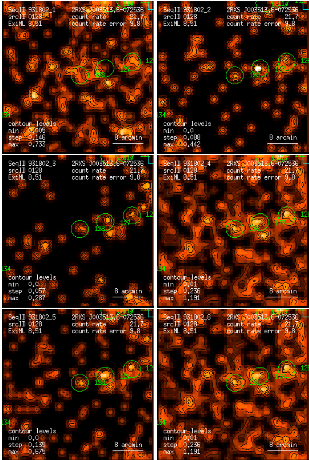
Figure 128: RASS 931802: detection 0128: band rate images, Gaussian filter: (1) PSPC channels 11 – 41, (2) 52 – 90, (3) 91 – 201, (4) 11 – 235, (5) 52 – 201, (6) 11 – 201. Broad band rates in counts/ks. Band rate contour levels in counts/ks/arcmin 2 .
