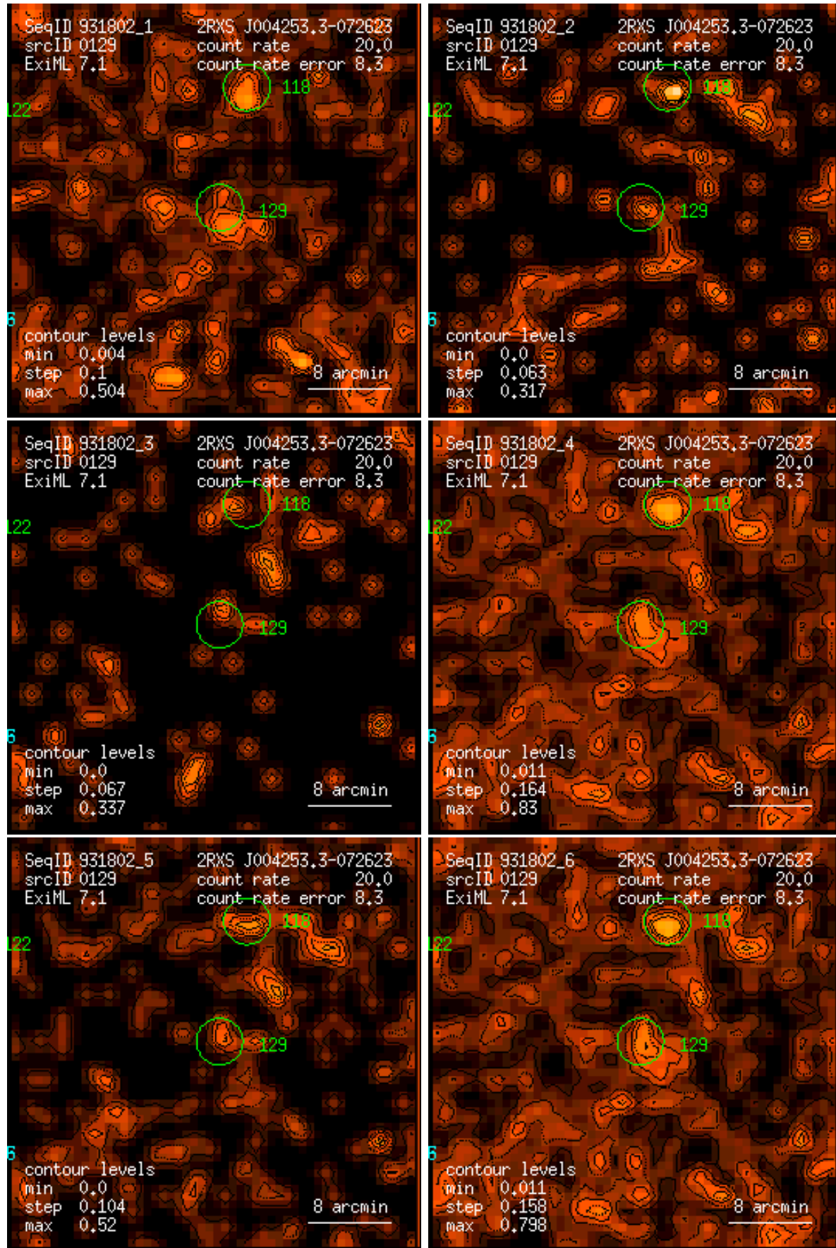
Figure 129: RASS 931802: detection 0129: band rate images, Gaussian filter: (1) PSPC channels 11 – 41, (2) 52 – 90, (3) 91 – 201, (4) 11 – 235, (5) 52 – 201, (6) 11 – 201. Broad band rates in counts/ks. Band rate contour levels in counts/ks/arcmin 2 .
