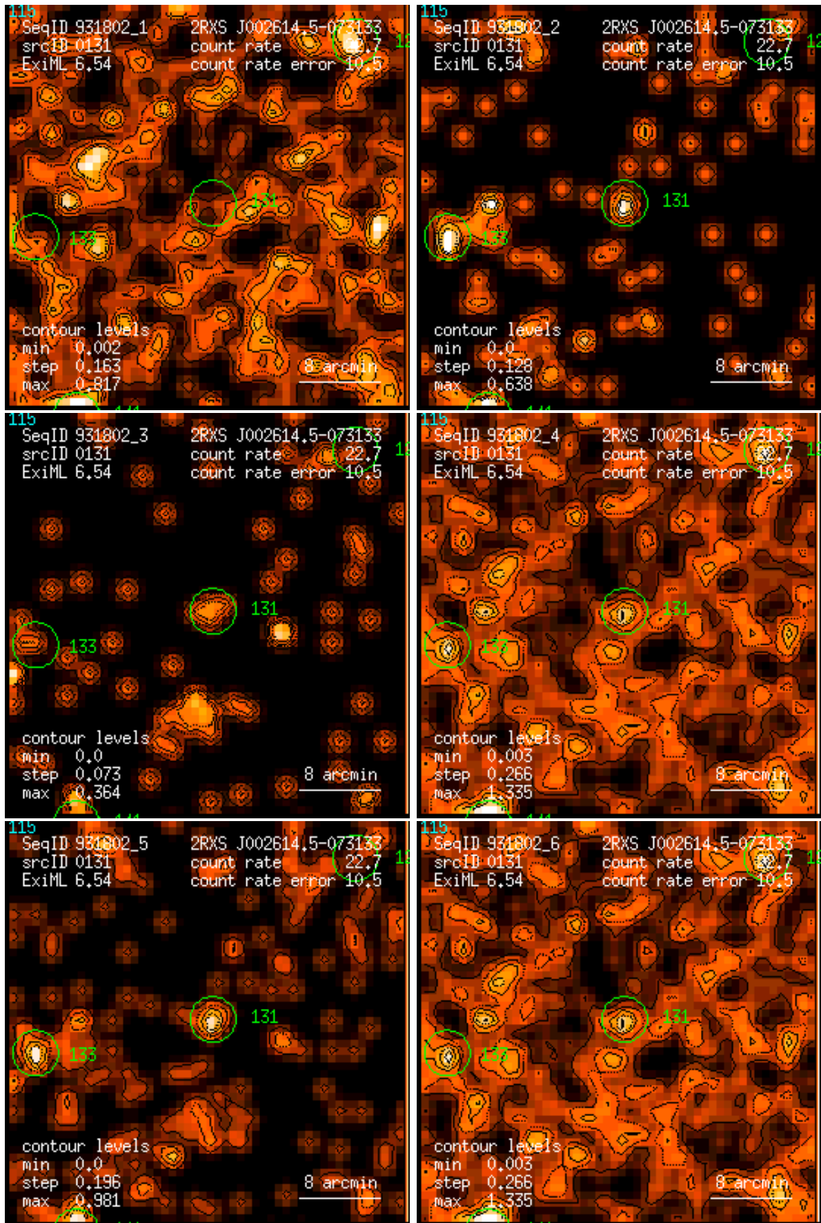
Figure 131: RASS 931802: detection 0131: band rate images, Gaussian filter: (1) PSPC channels 11 – 41, (2) 52 – 90, (3) 91 – 201, (4) 11 – 235, (5) 52 – 201, (6) 11 – 201. Broad band rates in counts/ks. Band rate contour levels in counts/ks/arcmin 2 .
