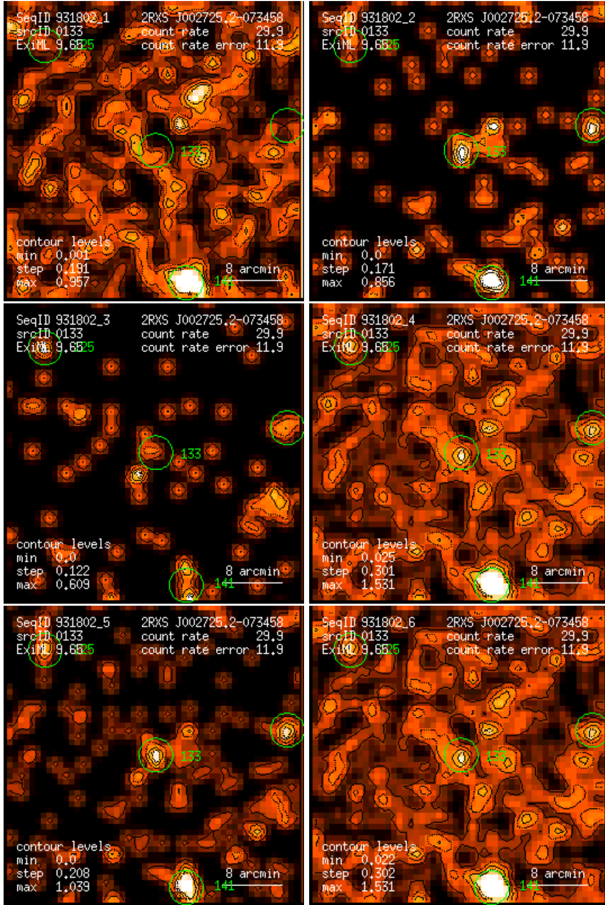
Figure 133: RASS 931802: detection 0133: band rate images, Gaussian filter: (1) PSPC channels 11 – 41, (2) 52 – 90, (3) 91 – 201, (4) 11 – 235, (5) 52 – 201, (6) 11 – 201. Broad band rates in counts/ks. Band rate contour levels in counts/ks/arcmin 2 .
