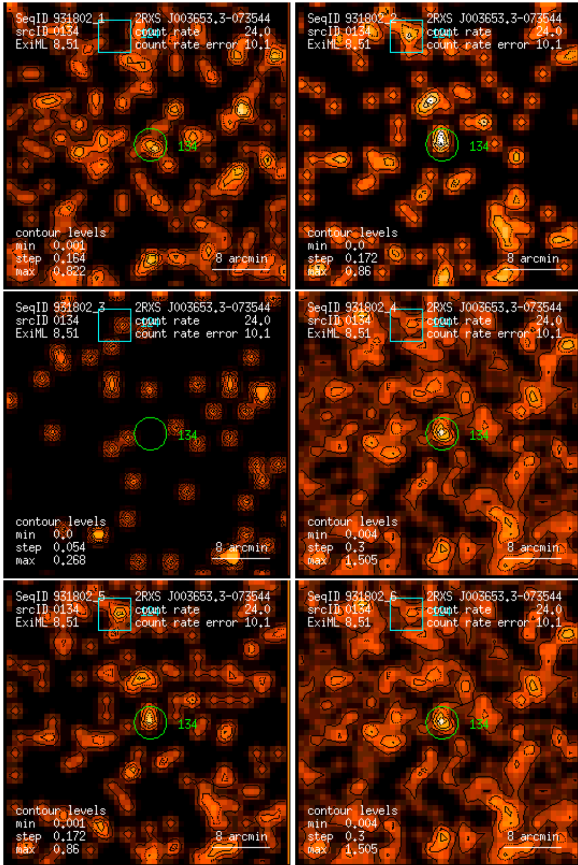
Figure 134: RASS 931802: detection 0134: band rate images, Gaussian filter: (1) PSPC channels 11 – 41, (2) 52 – 90, (3) 91 – 201, (4) 11 – 235, (5) 52 – 201, (6) 11 – 201. Broad band rates in counts/ks. Band rate contour levels in counts/ks/arcmin 2 .
