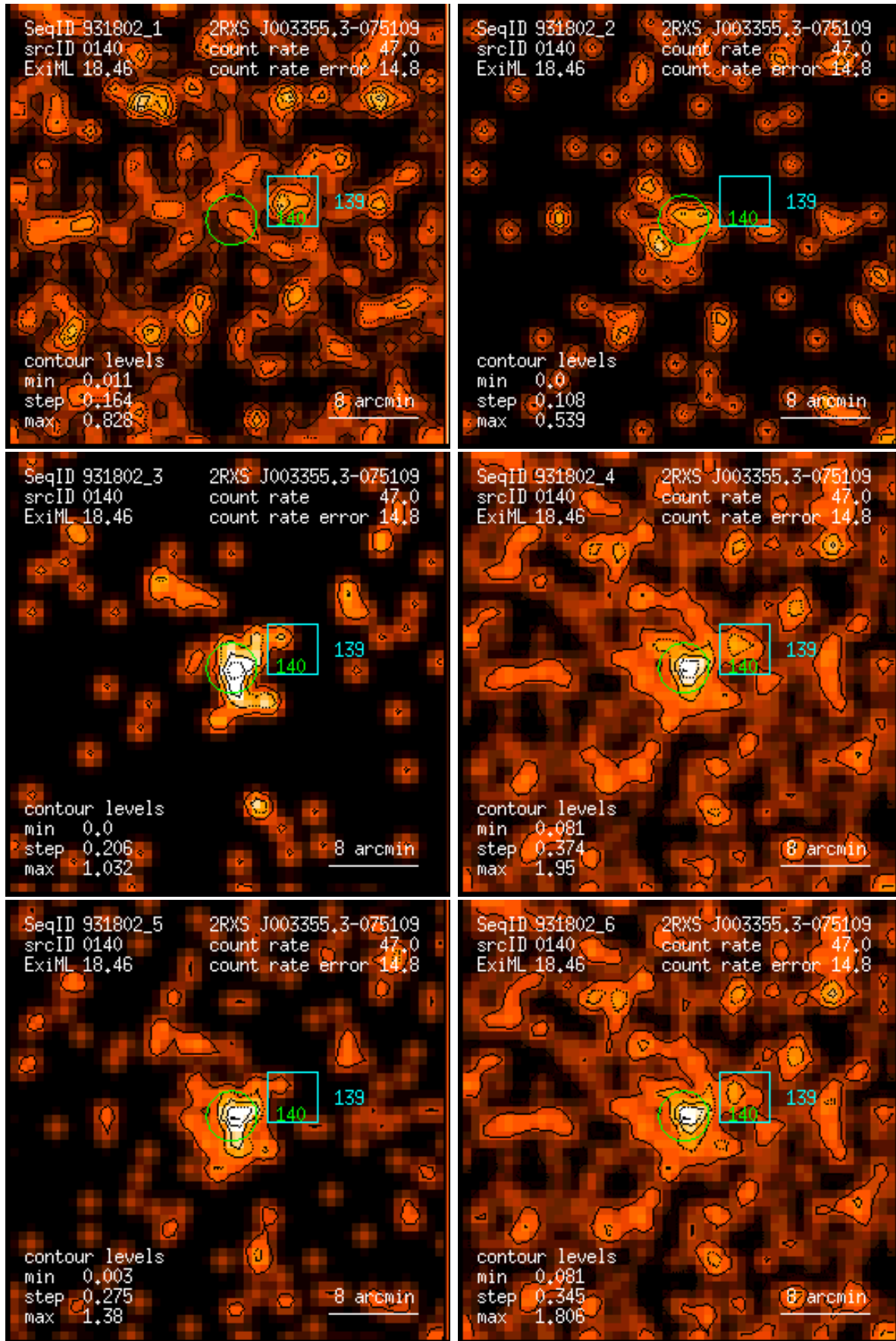
Figure 140: RASS 931802: detection 0140: band rate images, Gaussian filter: (1) PSPC channels 11 – 41, (2) 52 – 90, (3) 91 – 201, (4) 11 – 235, (5) 52 – 201, (6) 11 – 201. Broad band rates in counts/ks. Band rate contour levels in counts/ks/arcmin 2 .
