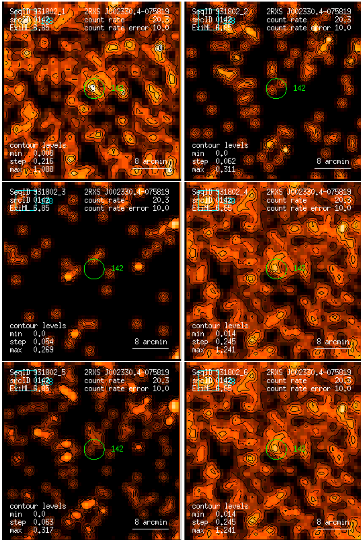
Figure 142: RASS 931802: detection 0142: band rate images, Gaussian filter: (1) PSPC channels 11 – 41, (2) 52 – 90, (3) 91 – 201, (4) 11 – 235, (5) 52 – 201, (6) 11 – 201. Broad band rates in counts/ks. Band rate contour levels in counts/ks/arcmin 2 .
