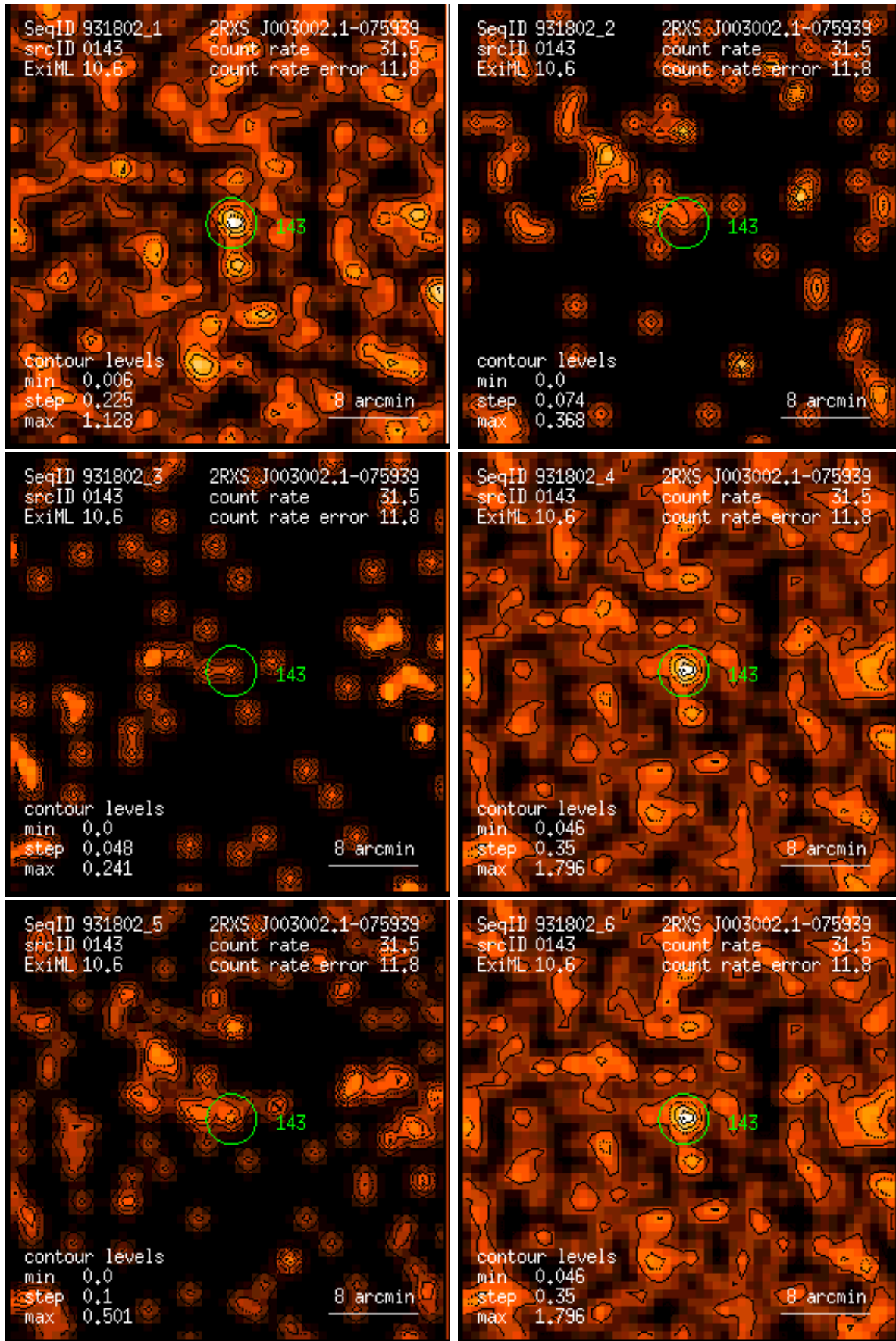
Figure 143: RASS 931802: detection 0143: band rate images, Gaussian filter: (1) PSPC channels 11 – 41, (2) 52 – 90, (3) 91 – 201, (4) 11 – 235, (5) 52 – 201, (6) 11 – 201. Broad band rates in counts/ks. Band rate contour levels in counts/ks/arcmin 2 .
