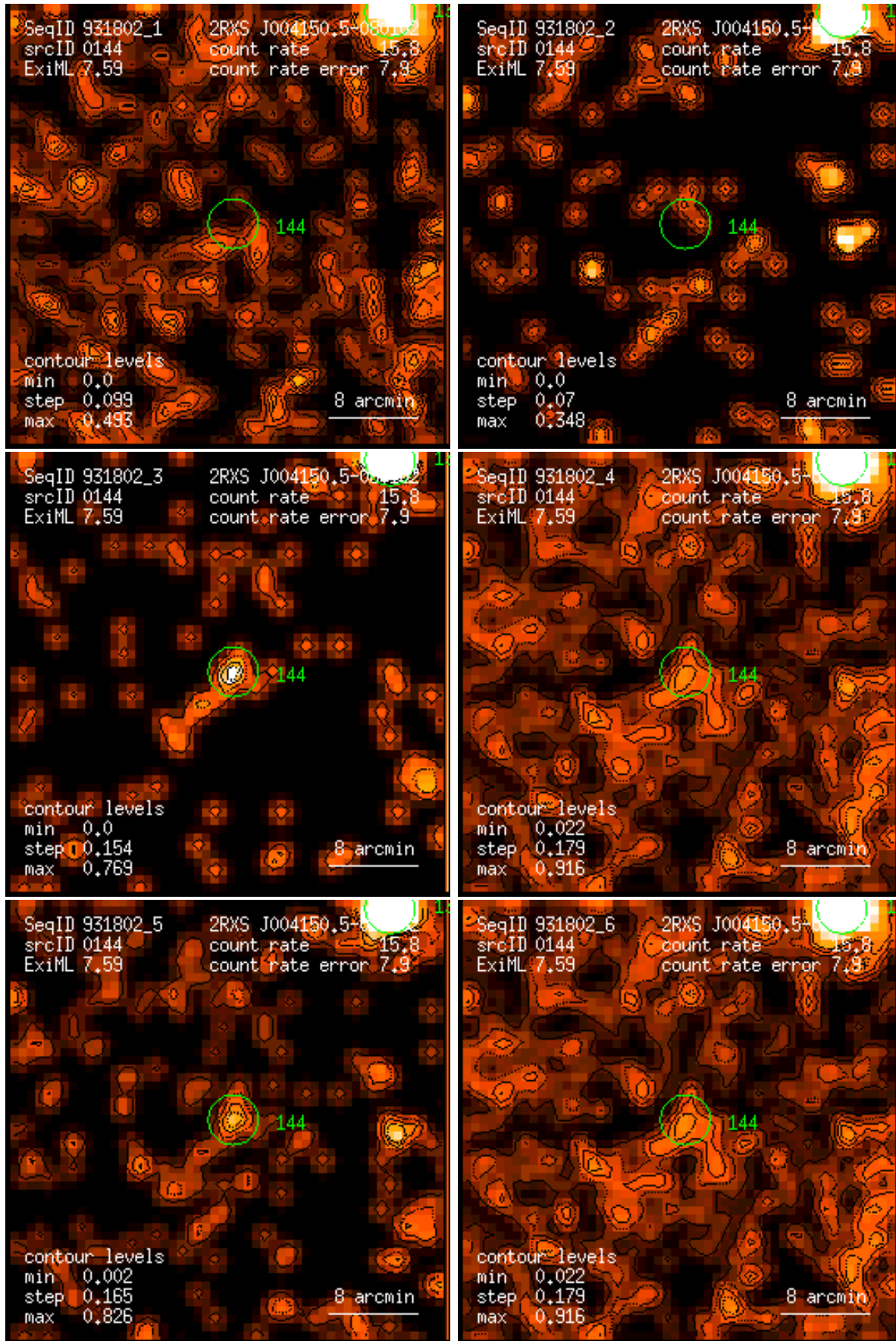
Figure 144: RASS 931802: detection 0144: band rate images, Gaussian filter: (1) PSPC channels 11 – 41, (2) 52 – 90, (3) 91 – 201, (4) 11 – 235, (5) 52 – 201, (6) 11 – 201. Broad band rates in counts/ks. Band rate contour levels in counts/ks/arcmin 2 .
