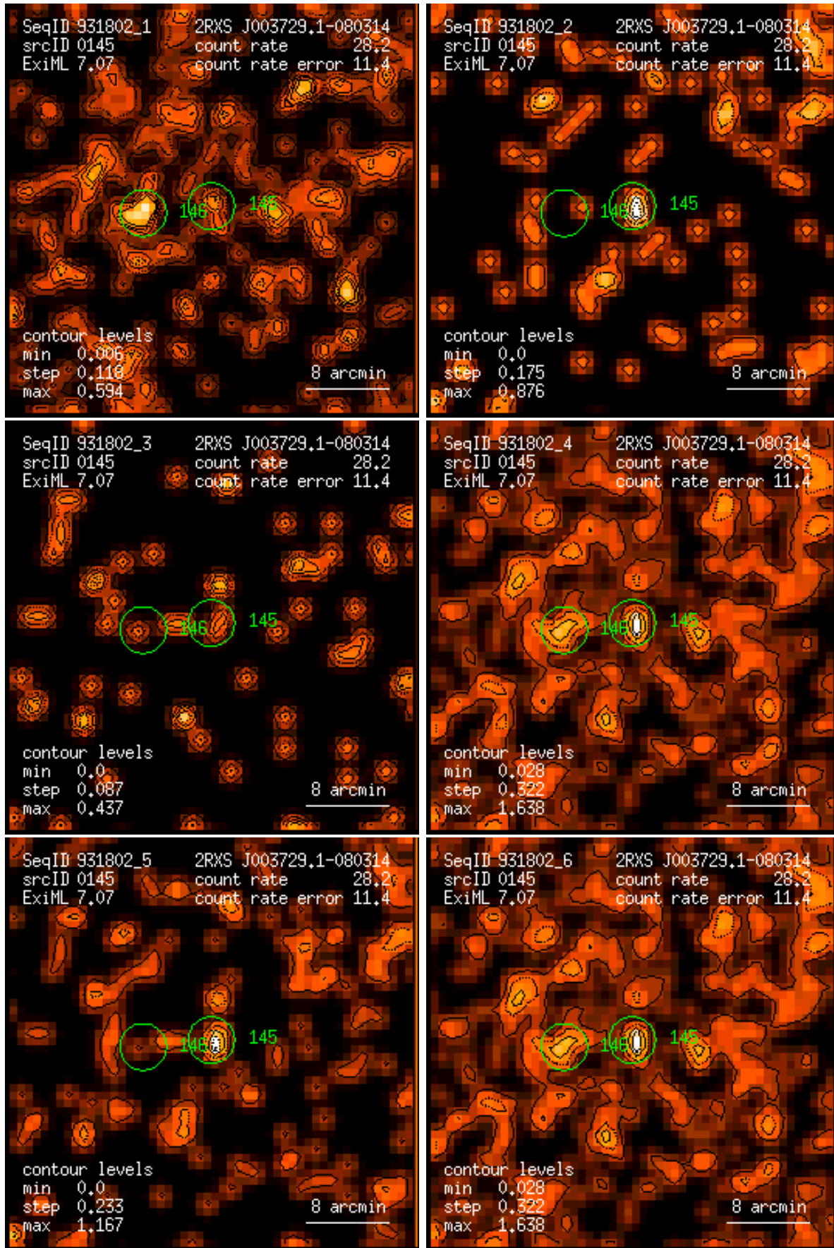
Figure 145: RASS 931802: detection 0145: band rate images, Gaussian filter: (1) PSPC channels 11 – 41, (2) 52 – 90, (3) 91 – 201, (4) 11 – 235, (5) 52 – 201, (6) 11 – 201. Broad band rates in counts/ks. Band rate contour levels in counts/ks/arcmin 2 .
