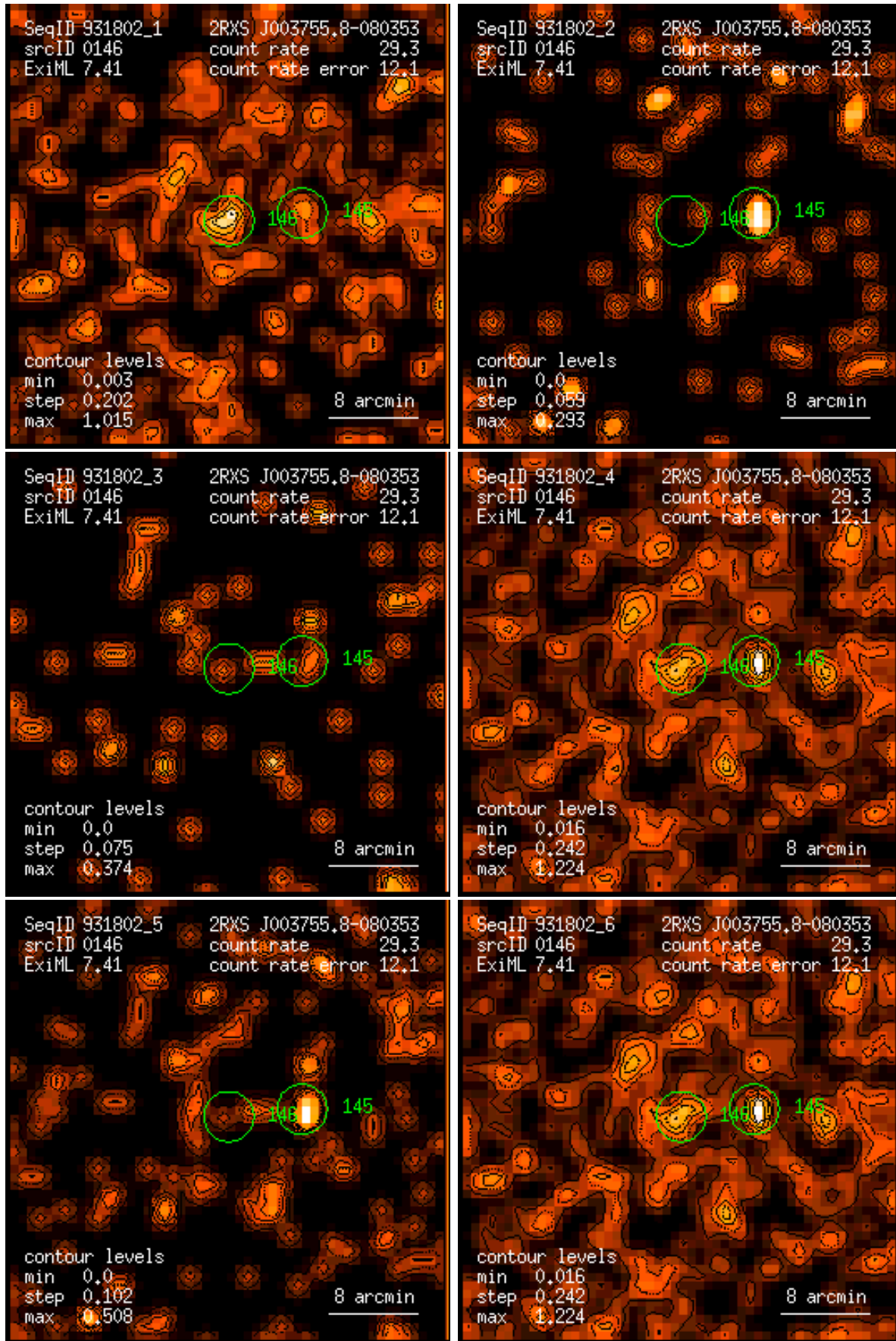
Figure 146: RASS 931802: detection 0146: band rate images, Gaussian filter: (1) PSPC channels 11 – 41, (2) 52 – 90, (3) 91 – 201, (4) 11 – 235, (5) 52 – 201, (6) 11 – 201. Broad band rates in counts/ks. Band rate contour levels in counts/ks/arcmin 2 .
