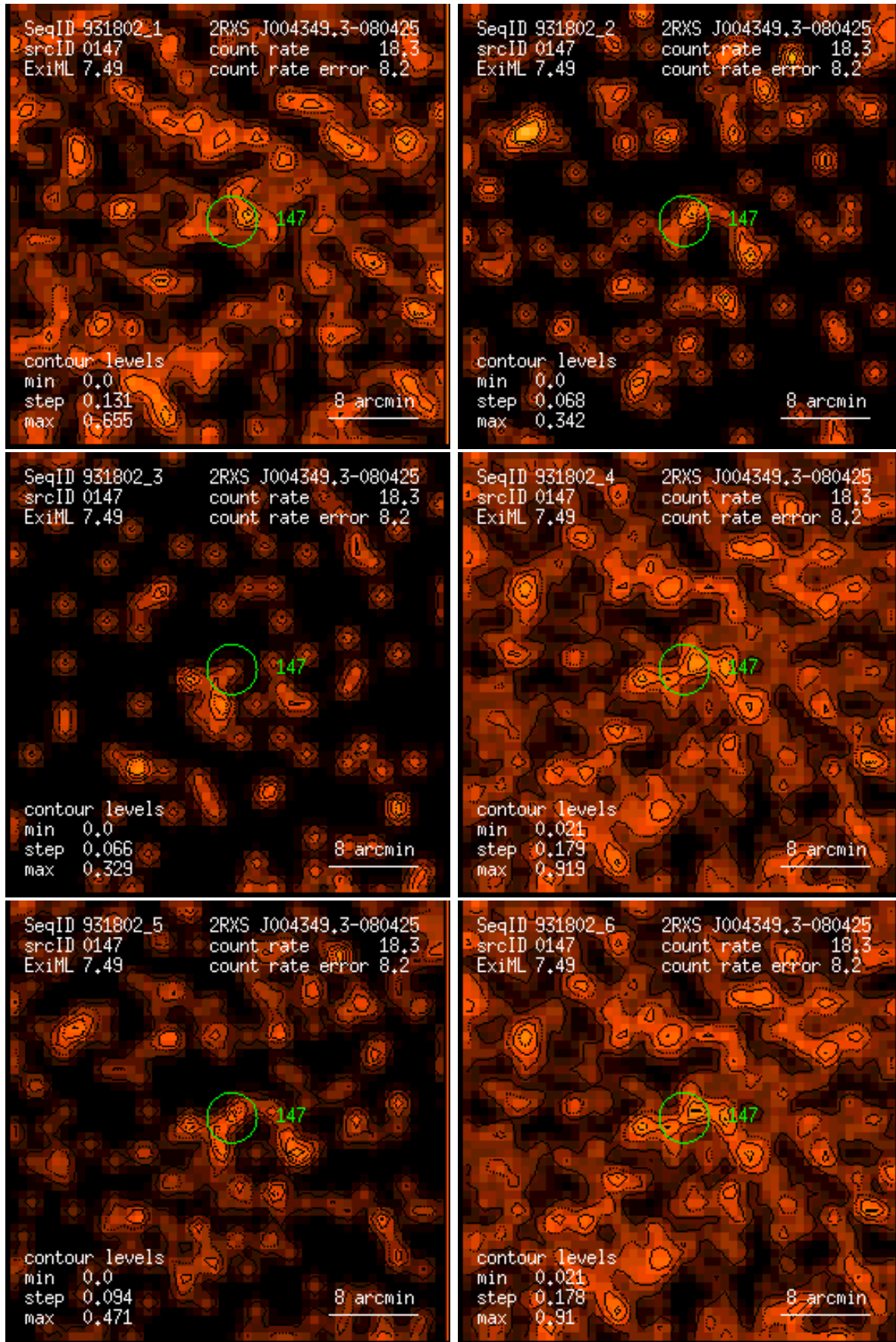
Figure 147: RASS 931802: detection 0147: band rate images, Gaussian filter: (1) PSPC channels 11 – 41, (2) 52 – 90, (3) 91 – 201, (4) 11 – 235, (5) 52 – 201, (6) 11 – 201. Broad band rates in counts/ks. Band rate contour levels in counts/ks/arcmin 2 .
