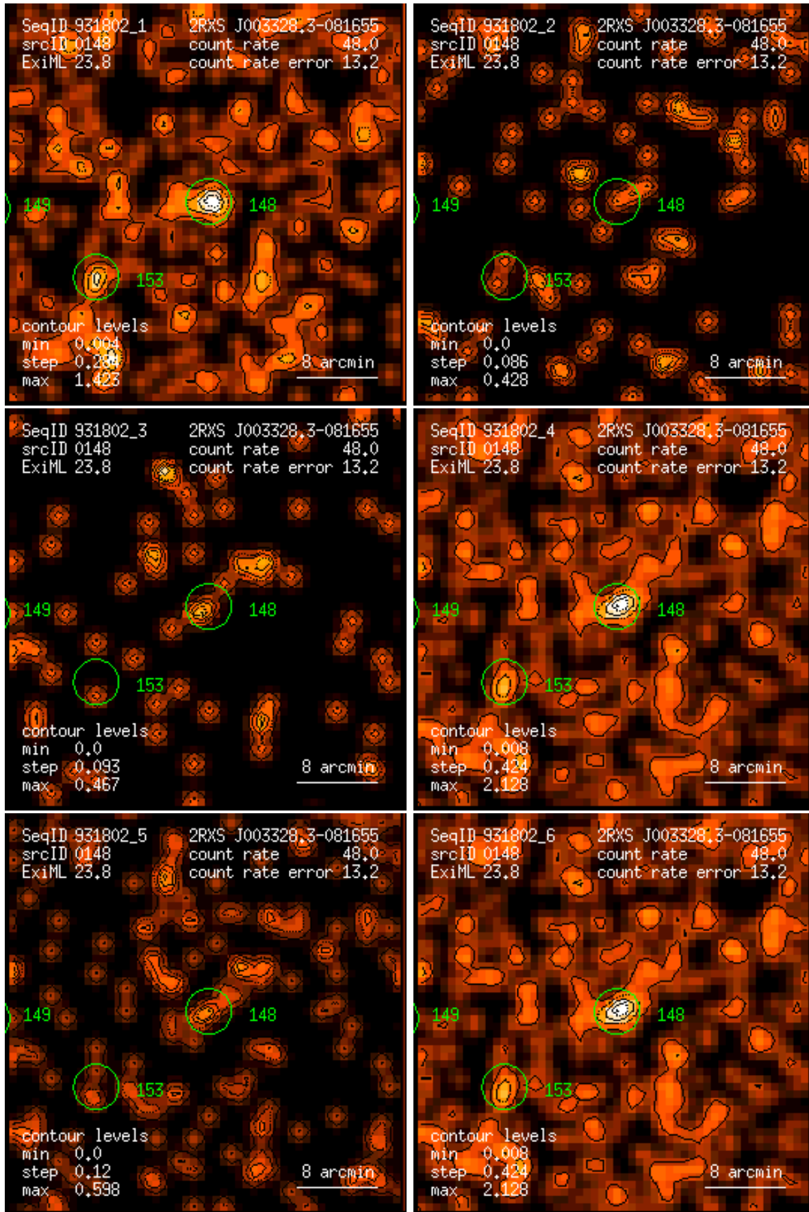
Figure 148: RASS 931802: detection 0148: band rate images, Gaussian filter: (1) PSPC channels 11 – 41, (2) 52 – 90, (3) 91 – 201, (4) 11 – 235, (5) 52 – 201, (6) 11 – 201. Broad band rates in counts/ks. Band rate contour levels in counts/ks/arcmin 2 .
