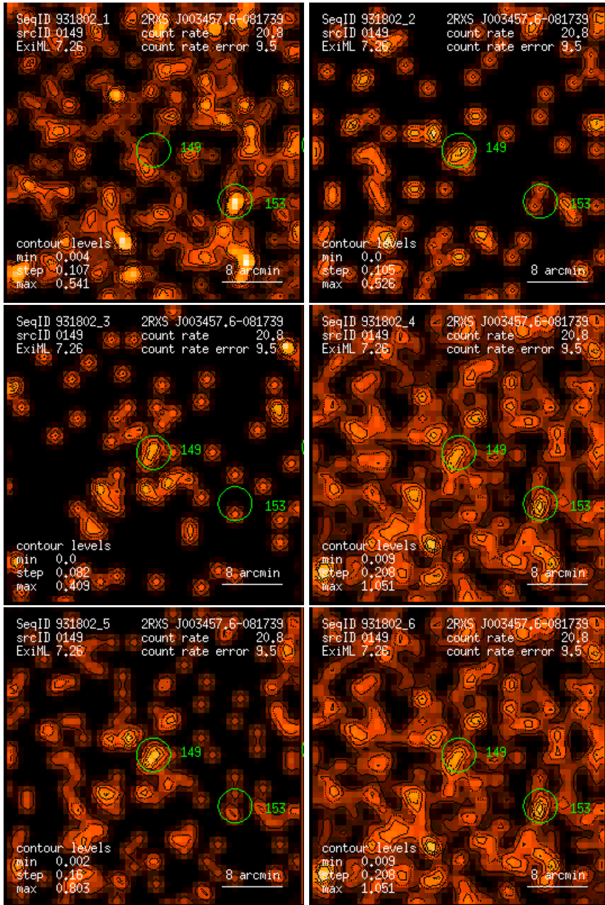
Figure 149: RASS 931802: detection 0149: band rate images, Gaussian filter: (1) PSPC channels 11 – 41, (2) 52 – 90, (3) 91 – 201, (4) 11 – 235, (5) 52 – 201, (6) 11 – 201. Broad band rates in counts/ks. Band rate contour levels in counts/ks/arcmin 2 .
