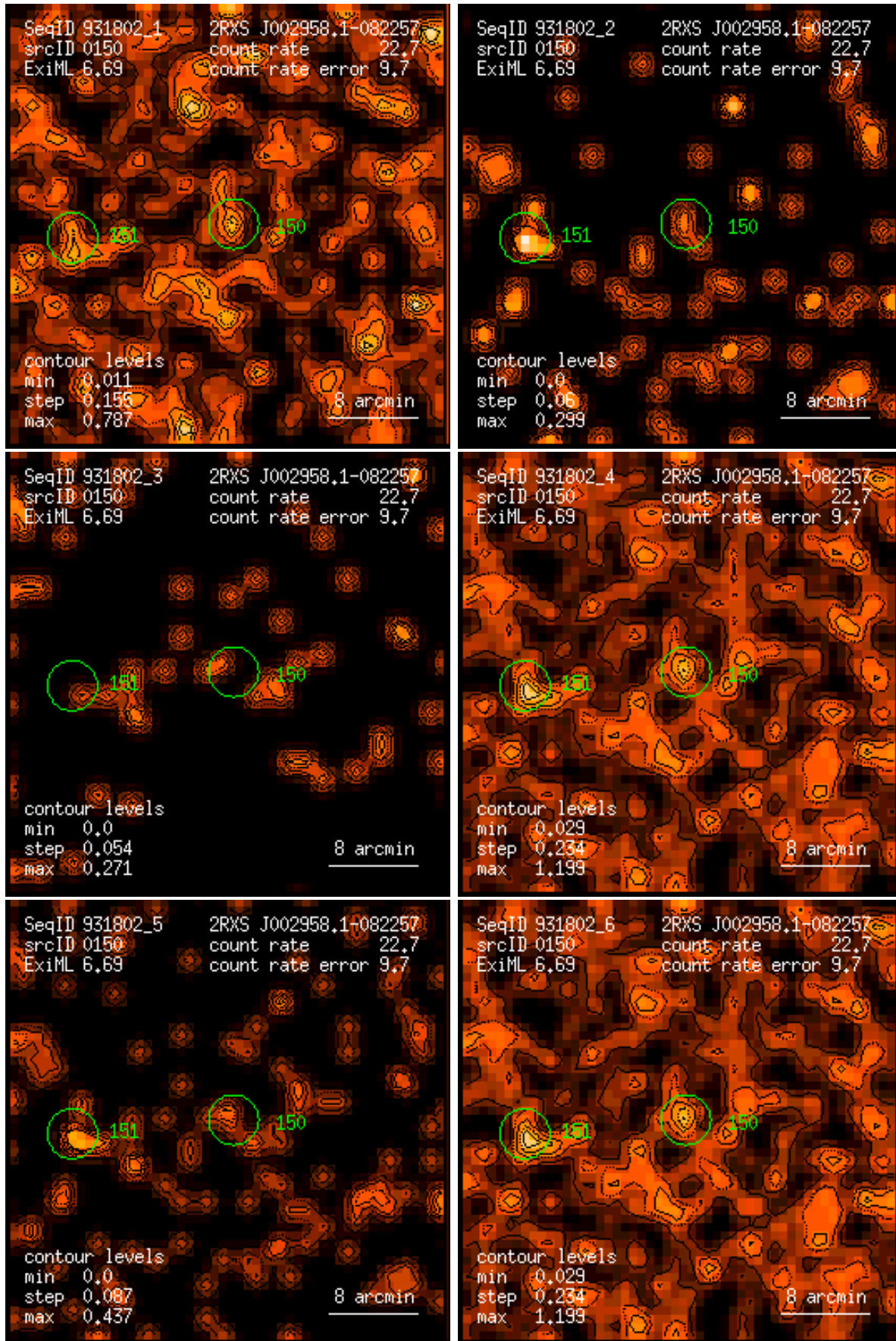
Figure 150: RASS 931802: detection 0150: band rate images, Gaussian filter: (1) PSPC channels 11 – 41, (2) 52 – 90, (3) 91 – 201, (4) 11 – 235, (5) 52 – 201, (6) 11 – 201. Broad band rates in counts/ks. Band rate contour levels in counts/ks/arcmin 2 .
