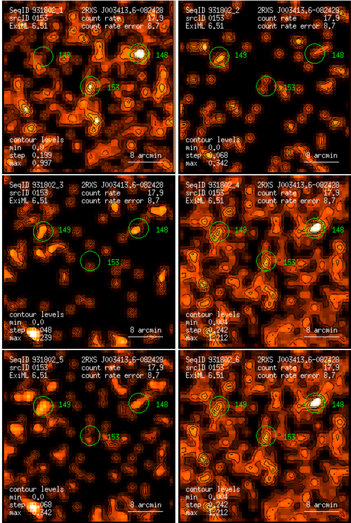
Figure 153: RASS 931802: detection 0153: band rate images, Gaussian filter: (1) PSPC channels 11 – 41, (2) 52 – 90, (3) 91 – 201, (4) 11 – 235, (5) 52 – 201, (6) 11 – 201. Broad band rates in counts/ks. Band rate contour levels in counts/ks/arcmin 2 .
