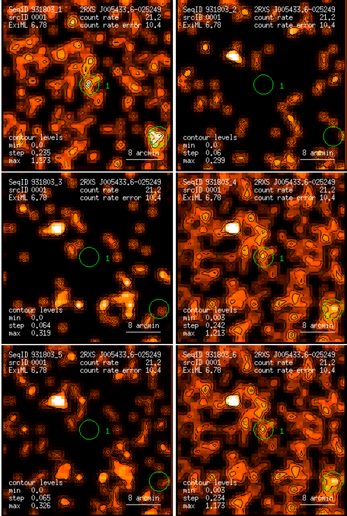
Figure 1: RASS 931803: detection 0001: band rate images, Gaussian filter: (1) PSPC channels 11 – 41, (2) 52 – 90, (3) 91 – 201, (4) 11 – 235, (5) 52 – 201, (6) 11 – 201. Broad band rates in counts/ks. Band rate contour levels in counts/ks/arcmin 2 .
