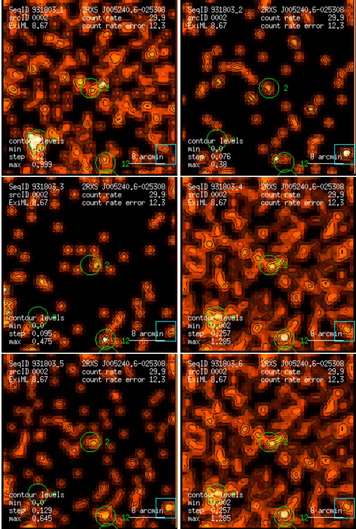
Figure 2: RASS 931803: detection 0002: band rate images, Gaussian filter: (1) PSPC channels 11 – 41, (2) 52 – 90, (3) 91 – 201, (4) 11 – 235, (5) 52 – 201, (6) 11 – 201. Broad band rates in counts/ks. Band rate contour levels in counts/ks/arcmin 2 .
