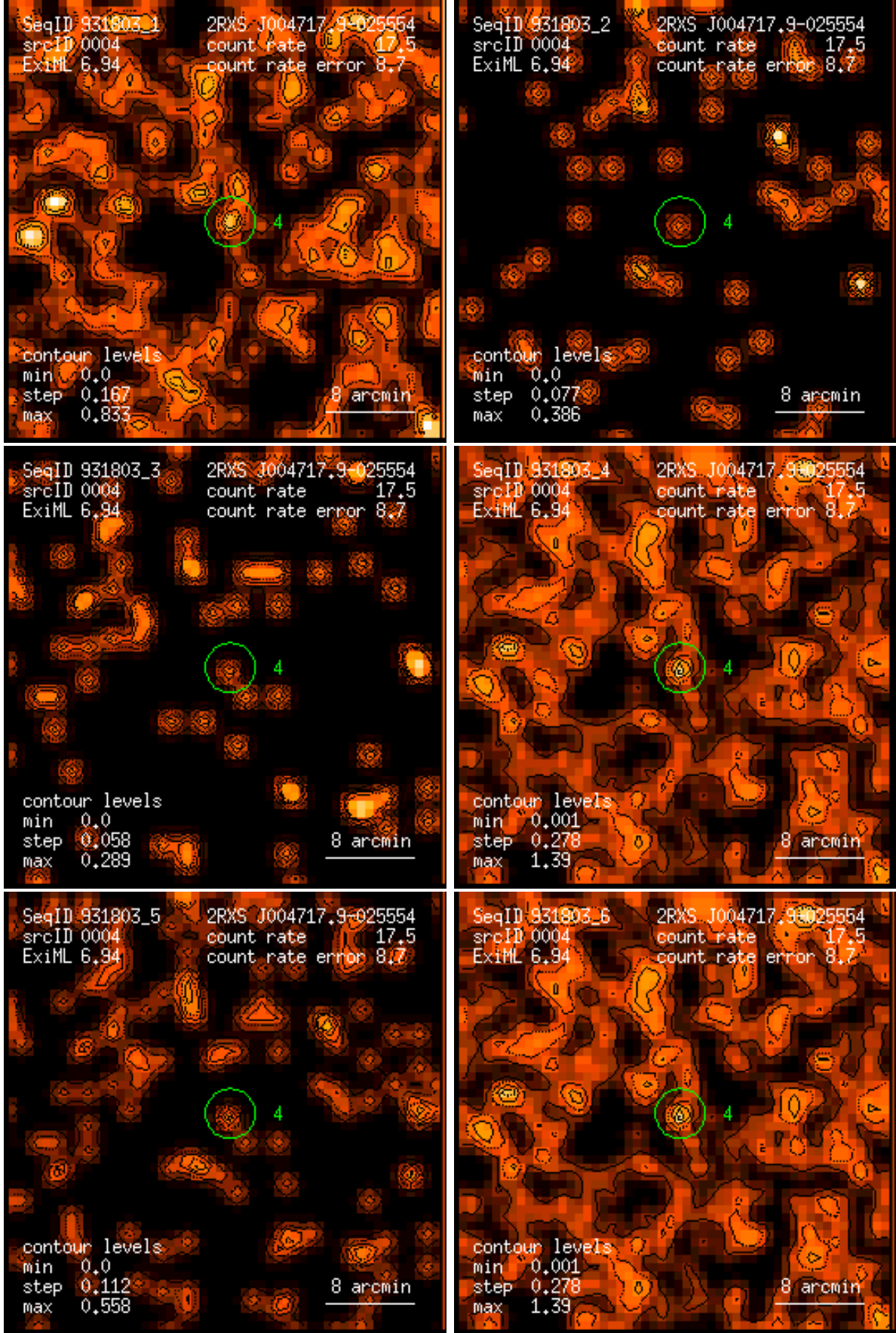
Figure 4: RASS 931803: detection 0004: band rate images, Gaussian filter: (1) PSPC channels 11 – 41, (2) 52 – 90, (3) 91 – 201, (4) 11 – 235, (5) 52 – 201, (6) 11 – 201. Broad band rates in counts/ks. Band rate contour levels in counts/ks/arcmin 2 .
