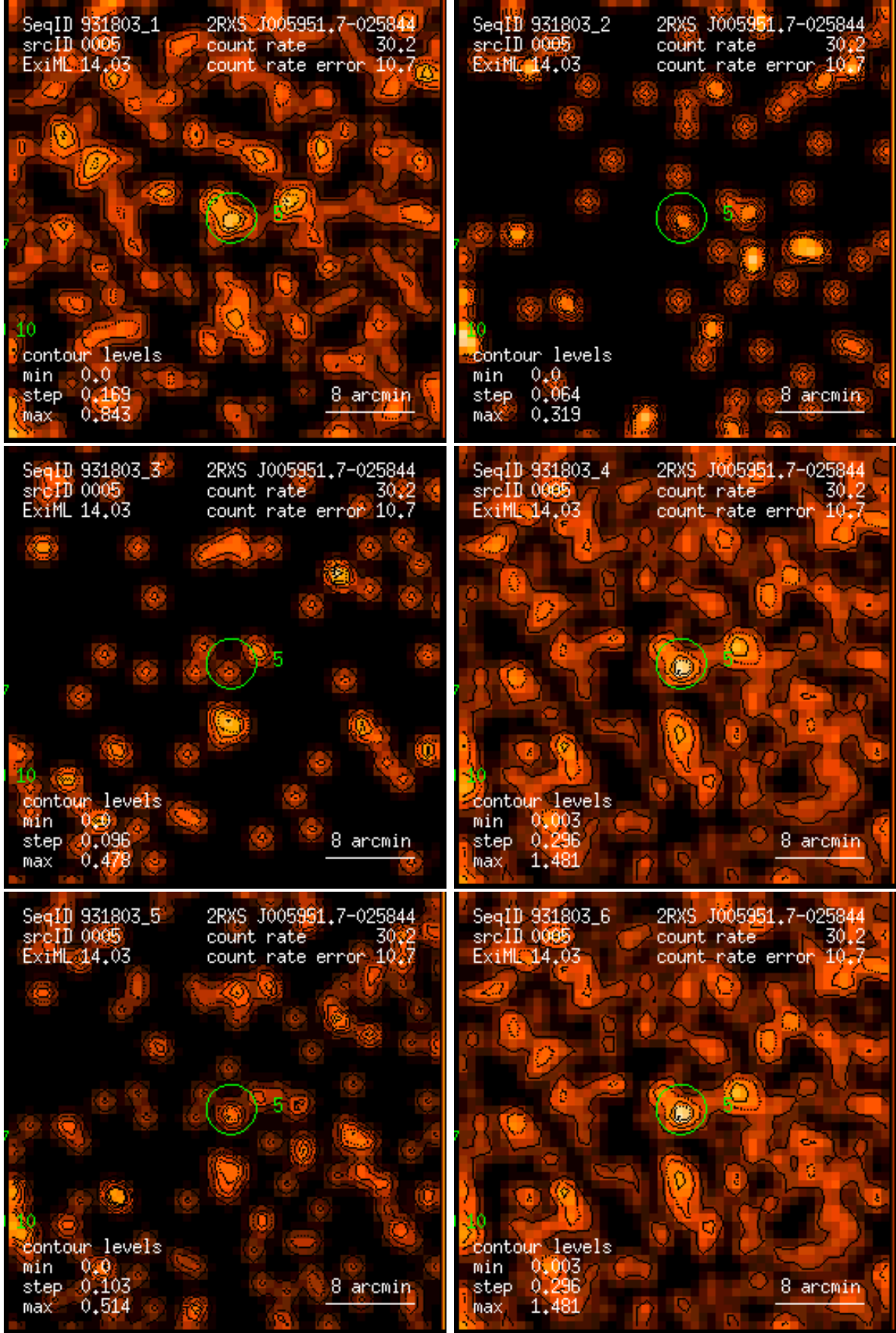
Figure 5: RASS 931803: detection 0005: band rate images, Gaussian filter: (1) PSPC channels 11 – 41, (2) 52 – 90, (3) 91 – 201, (4) 11 – 235, (5) 52 – 201, (6) 11 – 201. Broad band rates in counts/ks. Band rate contour levels in counts/ks/arcmin 2 .
