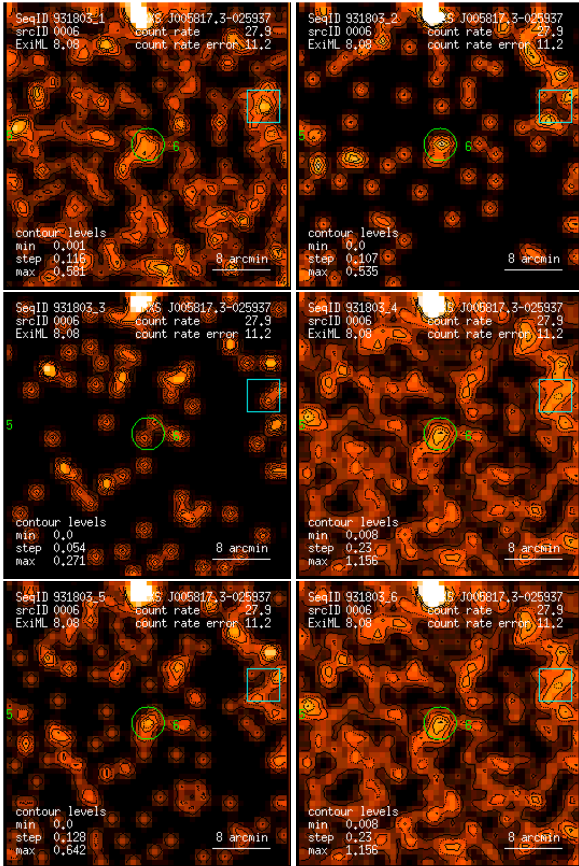
Figure 6: RASS 931803: detection 0006: band rate images, Gaussian filter: (1) PSPC channels 11 – 41, (2) 52 – 90, (3) 91 – 201, (4) 11 – 235, (5) 52 – 201, (6) 11 – 201. Broad band rates in counts/ks. Band rate contour levels in counts/ks/arcmin 2 .
