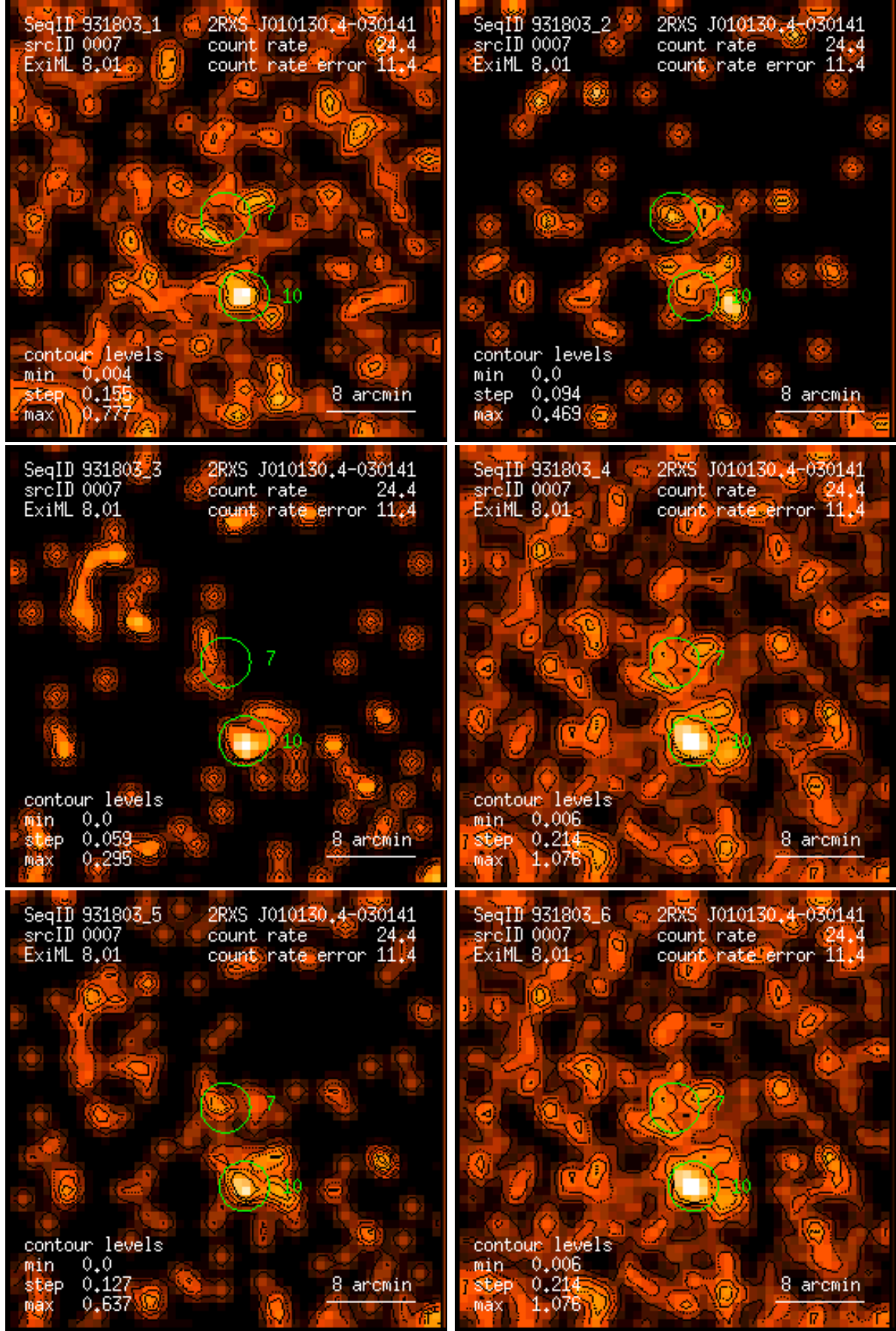
Figure 7: RASS 931803: detection 0007: band rate images, Gaussian filter: (1) PSPC channels 11 – 41, (2) 52 – 90, (3) 91 – 201, (4) 11 – 235, (5) 52 – 201, (6) 11 – 201. Broad band rates in counts/ks. Band rate contour levels in counts/ks/arcmin 2 .
