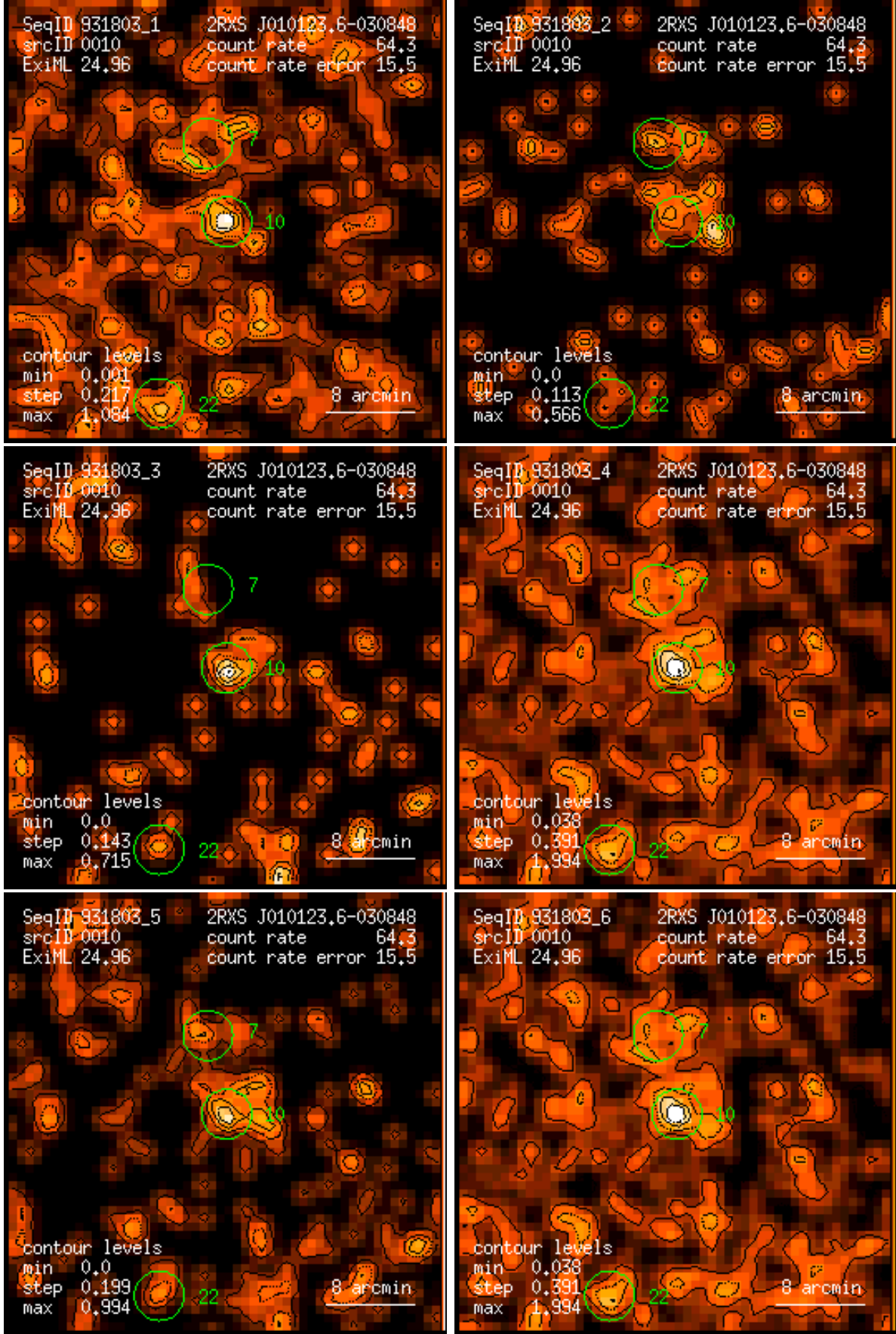
Figure 10: RASS 931803: detection 0010: band rate images, Gaussian filter: (1) PSPC channels 11 – 41, (2) 52 – 90, (3) 91 – 201, (4) 11 – 235, (5) 52 – 201, (6) 11 – 201. Broad band rates in counts/ks. Band rate contour levels in counts/ks/arcmin 2 .
