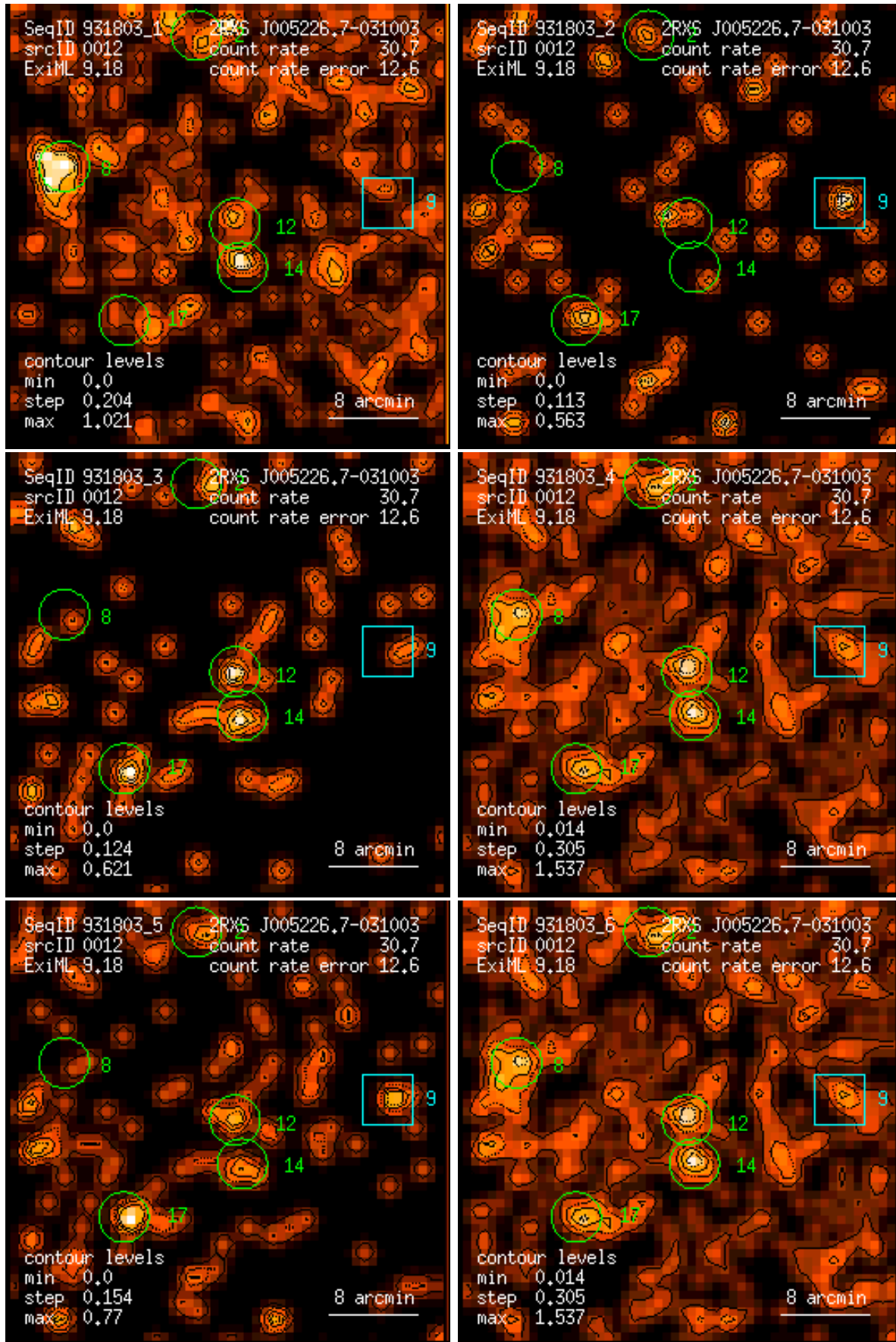
Figure 12: RASS 931803: detection 0012: band rate images, Gaussian filter: (1) PSPC channels 11 – 41, (2) 52 – 90, (3) 91 – 201, (4) 11 – 235, (5) 52 – 201, (6) 11 – 201. Broad band rates in counts/ks. Band rate contour levels in counts/ks/arcmin 2 .
