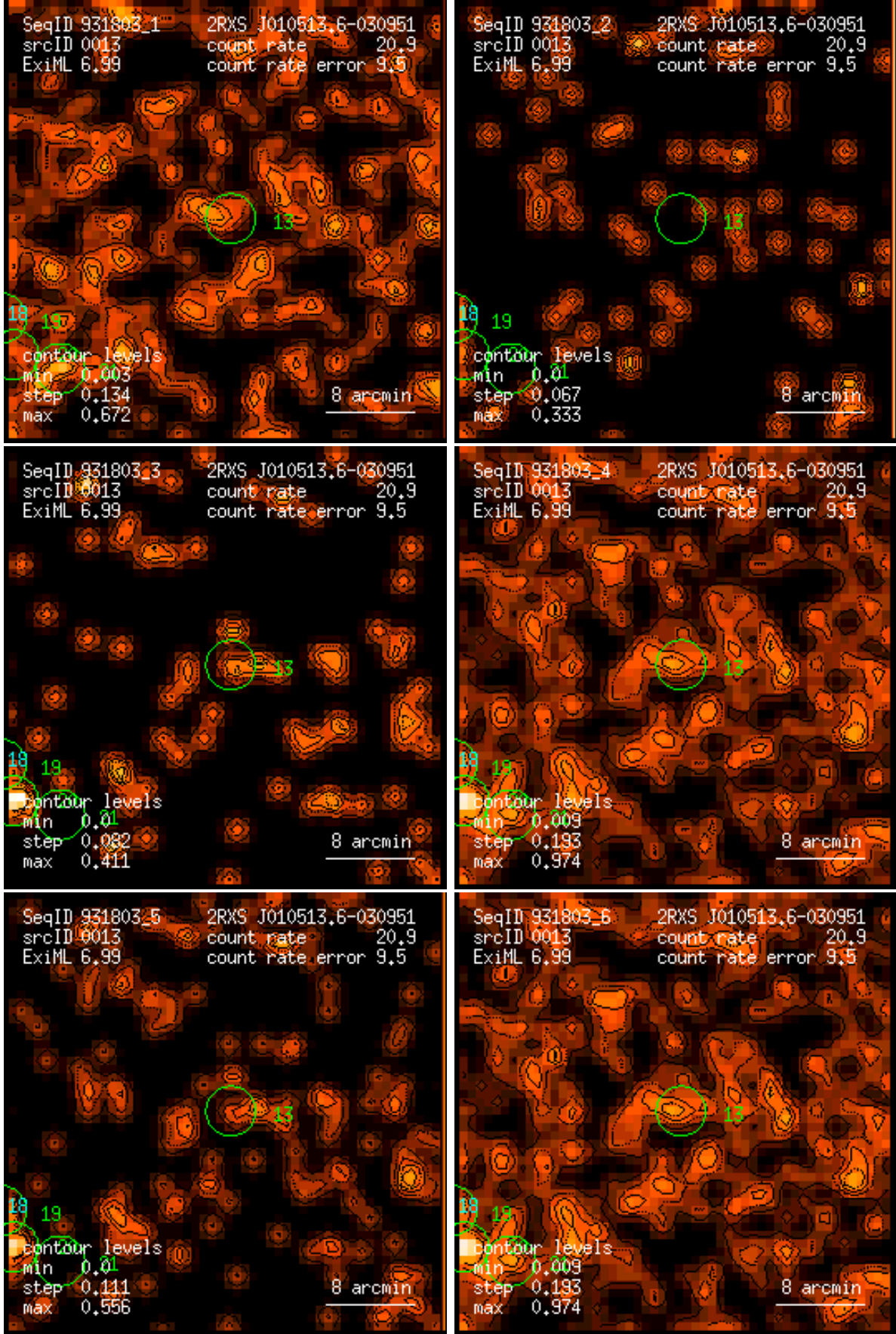
Figure 13: RASS 931803: detection 0013: band rate images, Gaussian filter: (1) PSPC channels 11 – 41, (2) 52 – 90, (3) 91 – 201, (4) 11 – 235, (5) 52 – 201, (6) 11 – 201. Broad band rates in counts/ks. Band rate contour levels in counts/ks/arcmin 2 .
