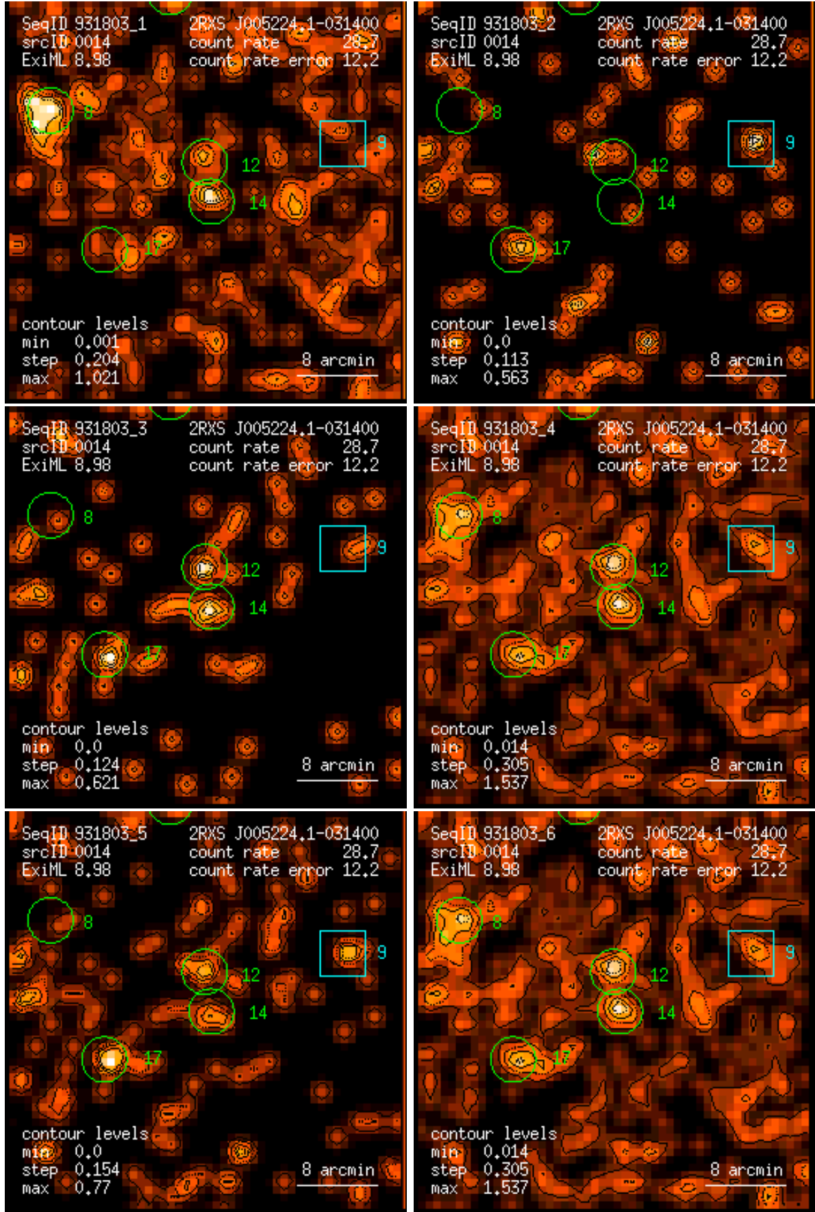
Figure 14: RASS 931803: detection 0014: band rate images, Gaussian filter: (1) PSPC channels 11 – 41, (2) 52 – 90, (3) 91 – 201, (4) 11 – 235, (5) 52 – 201, (6) 11 – 201. Broad band rates in counts/ks. Band rate contour levels in counts/ks/arcmin 2 .
