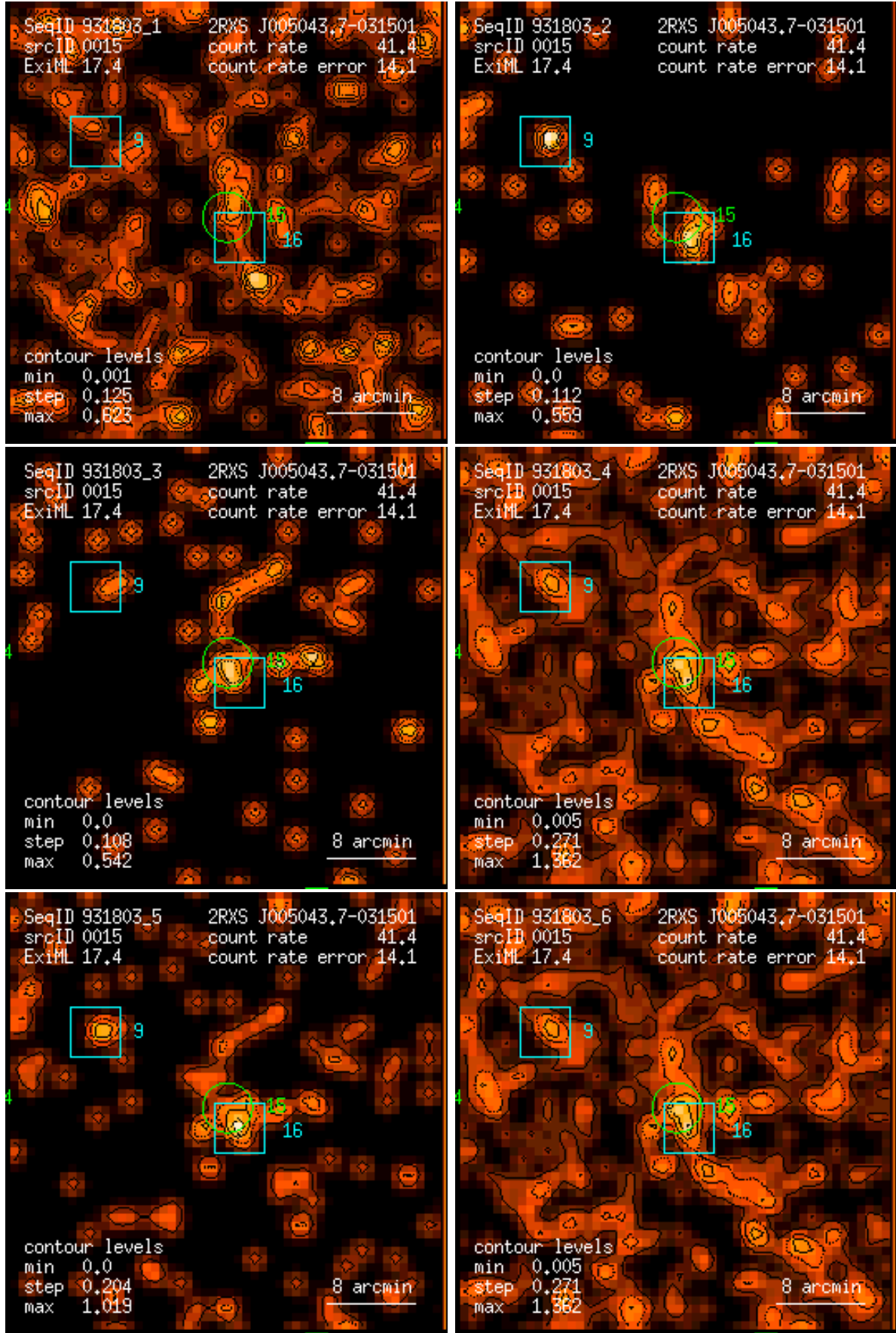
Figure 15: RASS 931803: detection 0015: band rate images, Gaussian filter: (1) PSPC channels 11 – 41, (2) 52 – 90, (3) 91 – 201, (4) 11 – 235, (5) 52 – 201, (6) 11 – 201. Broad band rates in counts/ks. Band rate contour levels in counts/ks/arcmin 2 .
