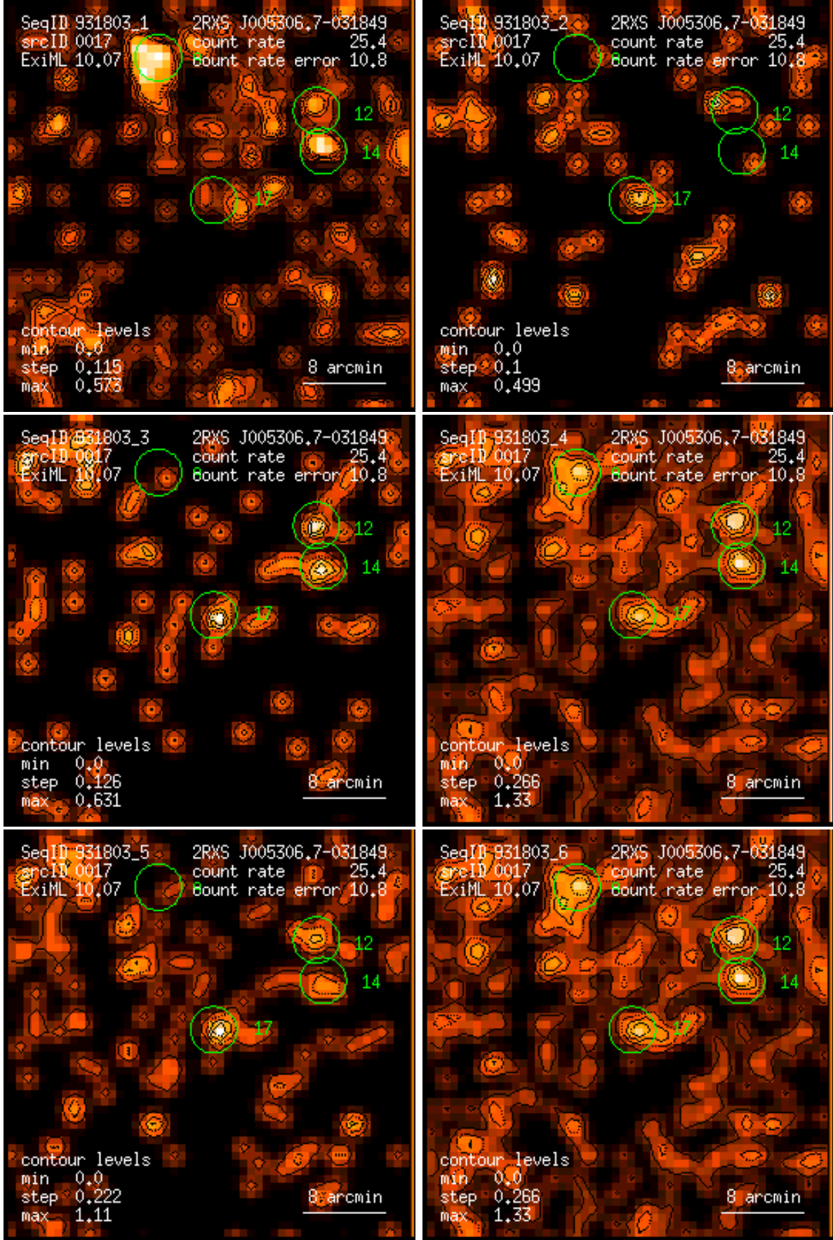
Figure 17: RASS 931803: detection 0017: band rate images, Gaussian filter: (1) PSPC channels 11 – 41, (2) 52 – 90, (3) 91 – 201, (4) 11 – 235, (5) 52 – 201, (6) 11 – 201. Broad band rates in counts/ks. Band rate contour levels in counts/ks/arcmin 2 .
