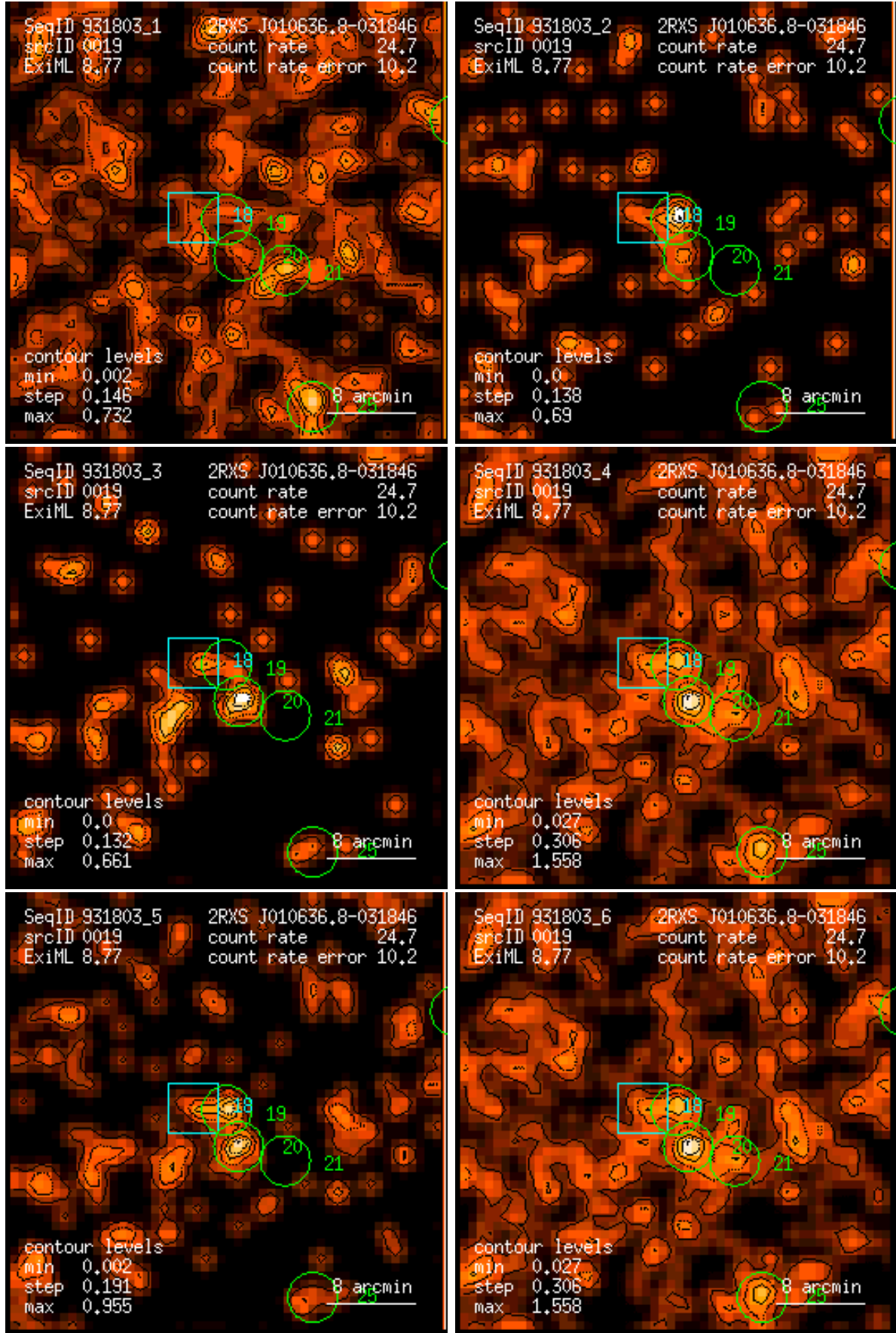
Figure 19: RASS 931803: detection 0019: band rate images, Gaussian filter: (1) PSPC channels 11 – 41, (2) 52 – 90, (3) 91 – 201, (4) 11 – 235, (5) 52 – 201, (6) 11 – 201. Broad band rates in counts/ks. Band rate contour levels in counts/ks/arcmin 2 .
