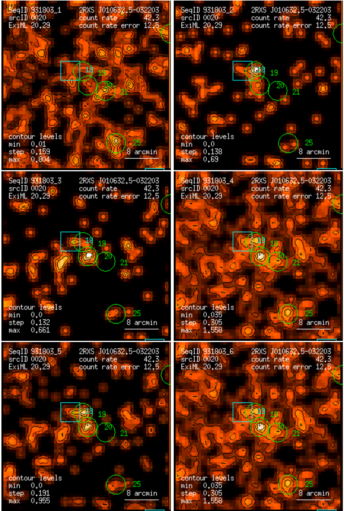
Figure 20: RASS 931803: detection 0020: band rate images, Gaussian filter: (1) PSPC channels 11 – 41, (2) 52 – 90, (3) 91 – 201, (4) 11 – 235, (5) 52 – 201, (6) 11 – 201. Broad band rates in counts/ks. Band rate contour levels in counts/ks/arcmin 2 .
