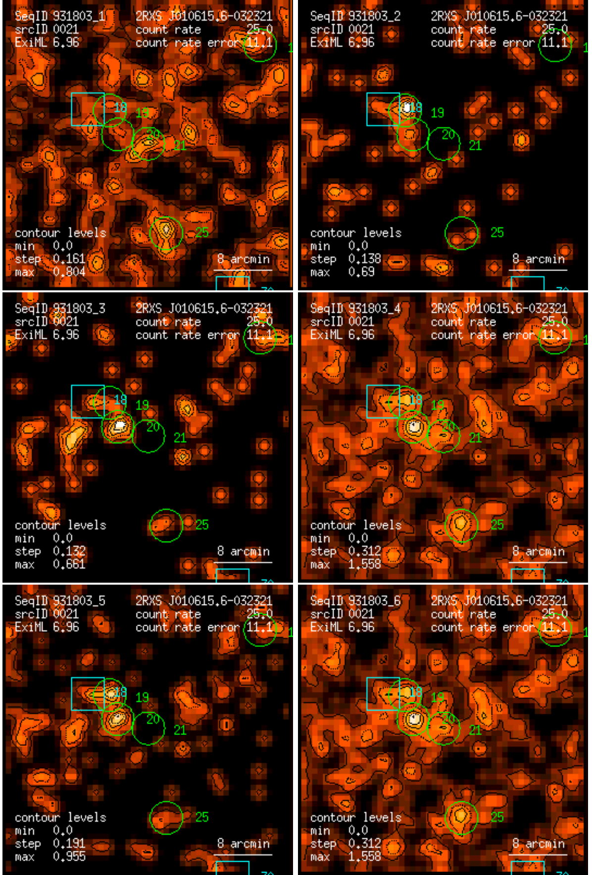
Figure 21: RASS 931803: detection 0021: band rate images, Gaussian filter: (1) PSPC channels 11 – 41, (2) 52 – 90, (3) 91 – 201, (4) 11 – 235, (5) 52 – 201, (6) 11 – 201. Broad band rates in counts/ks. Band rate contour levels in counts/ks/arcmin 2 .
