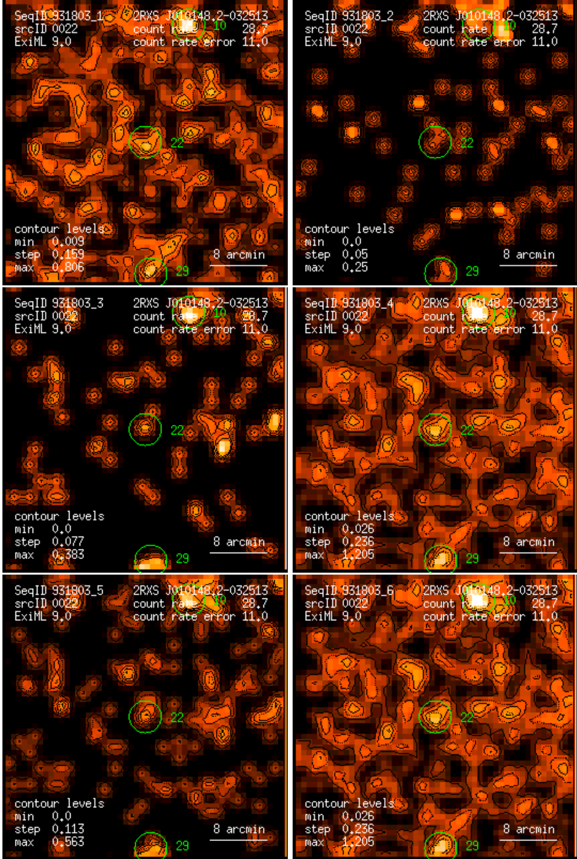
Figure 22: RASS 931803: detection 0022: band rate images, Gaussian filter: (1) PSPC channels 11 – 41, (2) 52 – 90, (3) 91 – 201, (4) 11 – 235, (5) 52 – 201, (6) 11 – 201. Broad band rates in counts/ks. Band rate contour levels in counts/ks/arcmin 2 .
