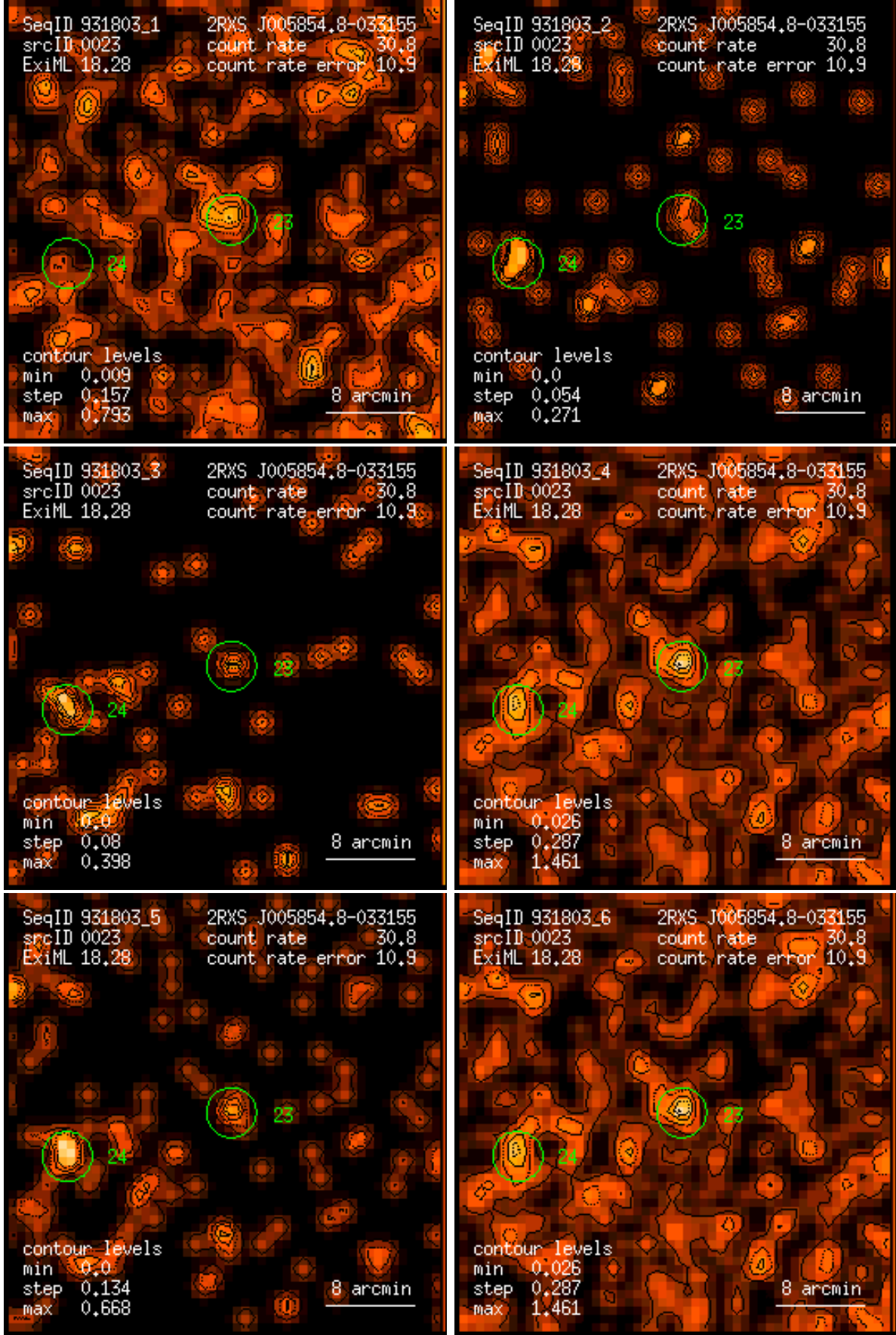
Figure 23: RASS 931803: detection 0023: band rate images, Gaussian filter: (1) PSPC channels 11 – 41, (2) 52 – 90, (3) 91 – 201, (4) 11 – 235, (5) 52 – 201, (6) 11 – 201. Broad band rates in counts/ks. Band rate contour levels in counts/ks/arcmin 2 .
