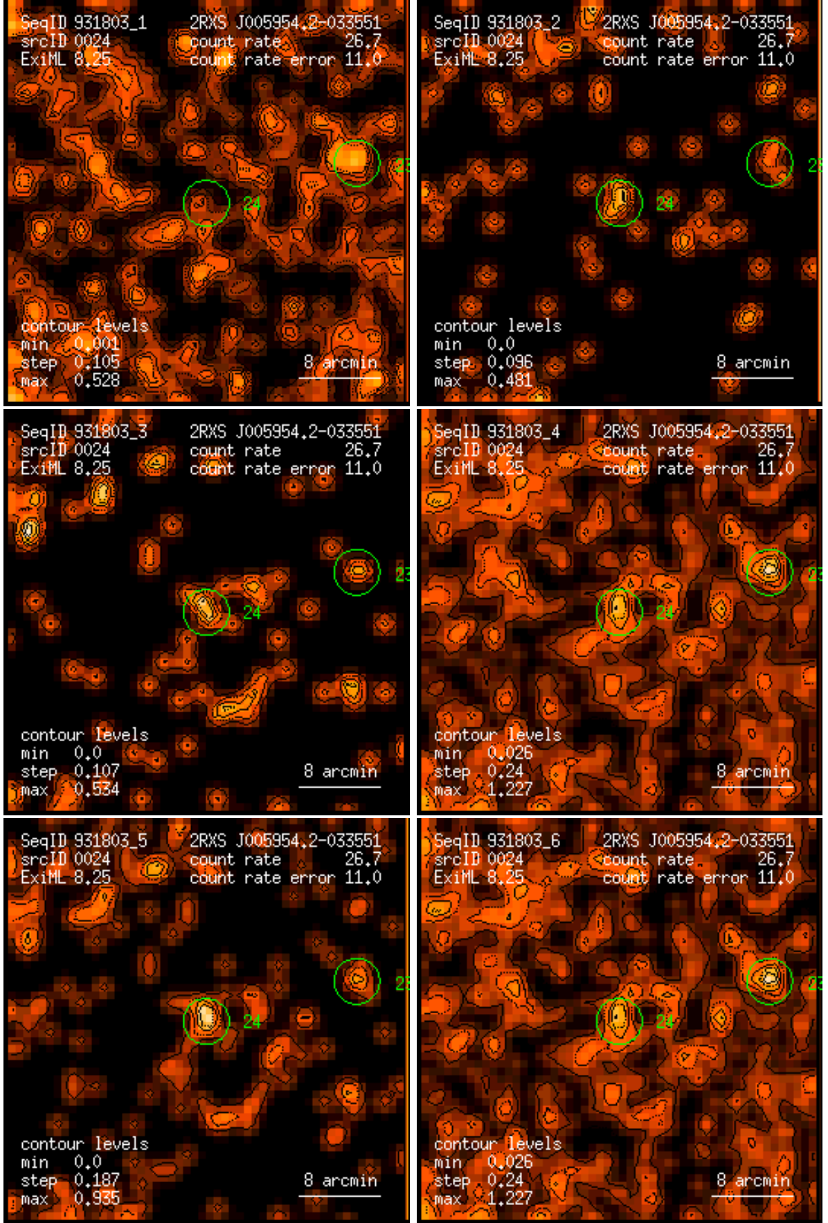
Figure 24: RASS 931803: detection 0024: band rate images, Gaussian filter: (1) PSPC channels 11 – 41, (2) 52 – 90, (3) 91 – 201, (4) 11 – 235, (5) 52 – 201, (6) 11 – 201. Broad band rates in counts/ks. Band rate contour levels in counts/ks/arcmin 2 .
