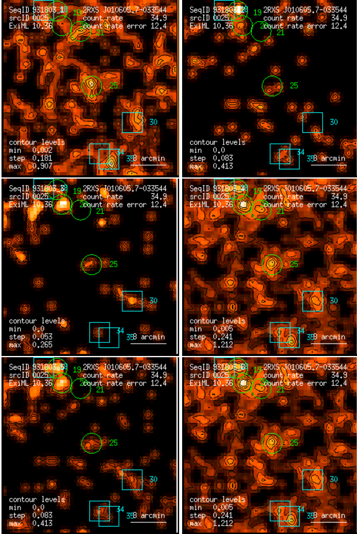
Figure 25: RASS 931803: detection 0025: band rate images, Gaussian filter: (1) PSPC channels 11 – 41, (2) 52 – 90, (3) 91 – 201, (4) 11 – 235, (5) 52 – 201, (6) 11 – 201. Broad band rates in counts/ks. Band rate contour levels in counts/ks/arcmin 2 .
