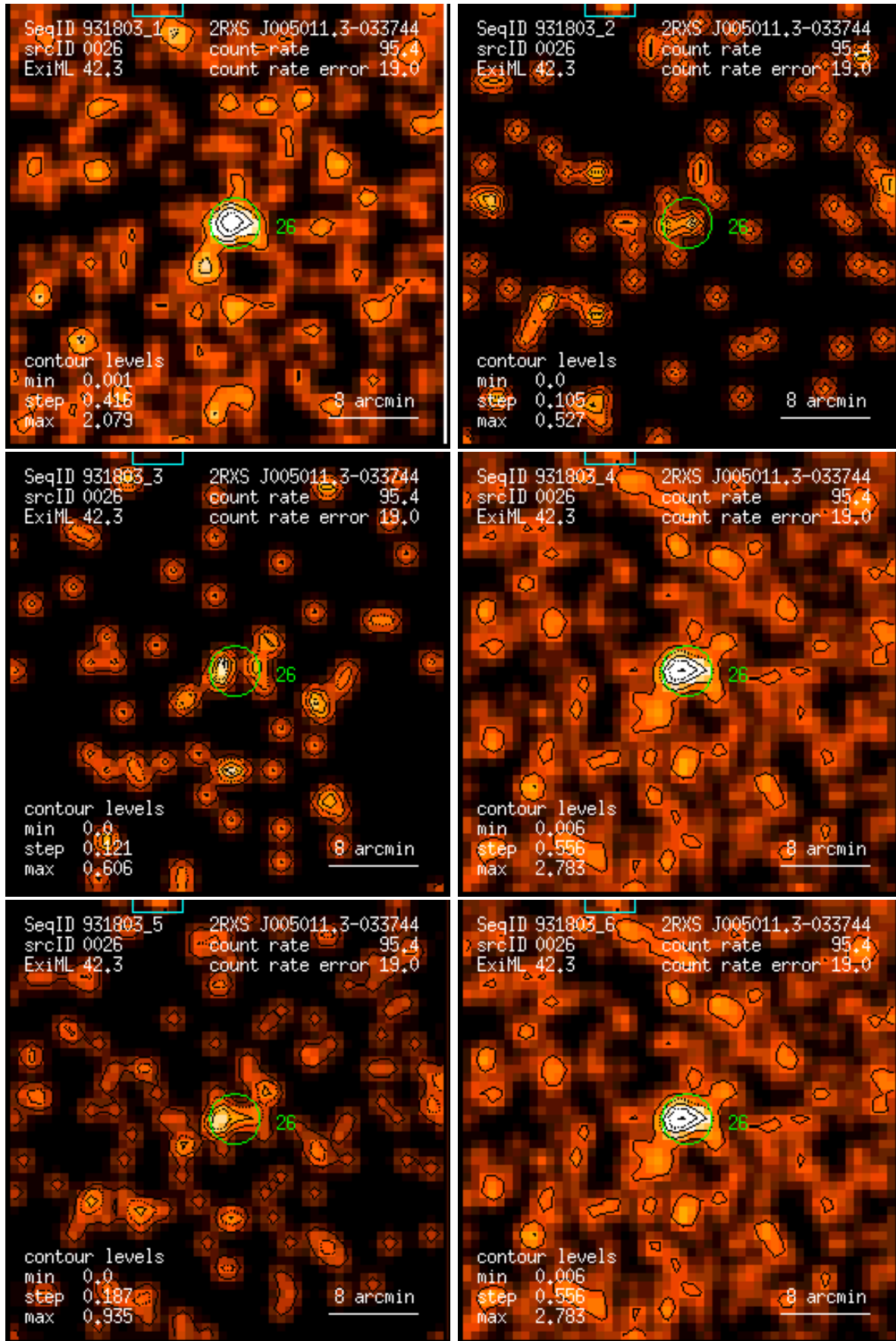
Figure 26: RASS 931803: detection 0026: band rate images, Gaussian filter: (1) PSPC channels 11 – 41, (2) 52 – 90, (3) 91 – 201, (4) 11 – 235, (5) 52 – 201, (6) 11 – 201. Broad band rates in counts/ks. Band rate contour levels in counts/ks/arcmin 2 .
