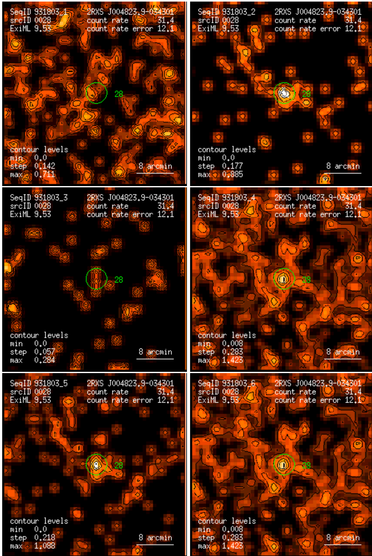
Figure 28: RASS 931803: detection 0028: band rate images, Gaussian filter: (1) PSPC channels 11 – 41, (2) 52 – 90, (3) 91 – 201, (4) 11 – 235, (5) 52 – 201, (6) 11 – 201. Broad band rates in counts/ks. Band rate contour levels in counts/ks/arcmin 2 .
