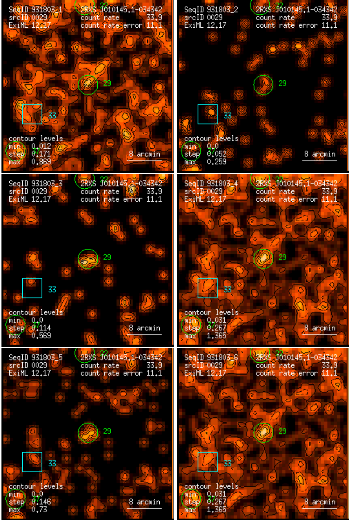
Figure 29: RASS 931803: detection 0029: band rate images, Gaussian filter: (1) PSPC channels 11 – 41, (2) 52 – 90, (3) 91 – 201, (4) 11 – 235, (5) 52 – 201, (6) 11 – 201. Broad band rates in counts/ks. Band rate contour levels in counts/ks/arcmin 2 .
