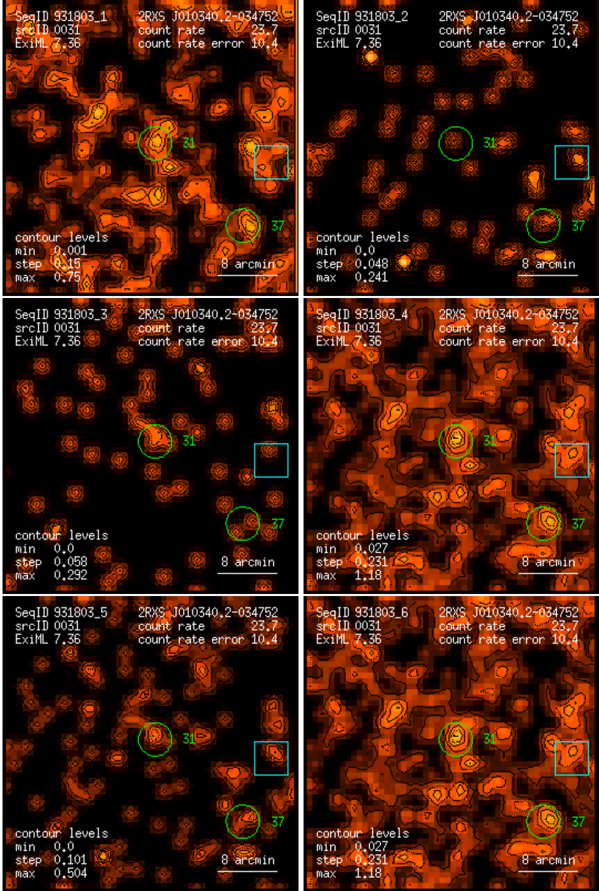
Figure 31: RASS 931803: detection 0031: band rate images, Gaussian filter: (1) PSPC channels 11 – 41, (2) 52 – 90, (3) 91 – 201, (4) 11 – 235, (5) 52 – 201, (6) 11 – 201. Broad band rates in counts/ks. Band rate contour levels in counts/ks/arcmin 2 .
